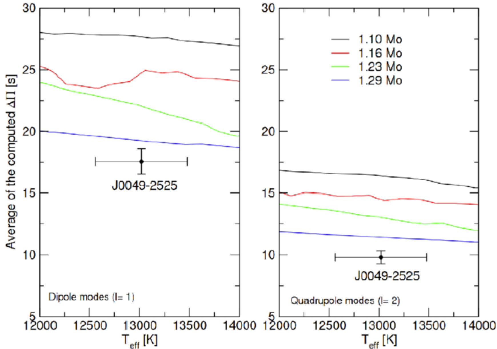
Figure 8. from Ozcan Caliskan et al 2025 Astrophys. J. 988 doi:10.3847/1538-4357/addc70 https://dx.doi.org/10.3847/1538-4357/addc70 © 2025. The Author(s). Published by the American Astronomical Society.
