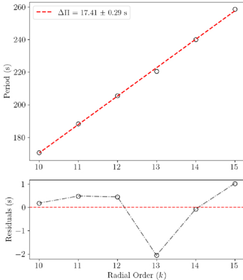
Figure 7. from Ozcan Caliskan et al 2025 Astrophys. J. 988 doi:10.3847/1538-4357/addc70 https://dx.doi.org/10.3847/1538-4357/addc70 © 2025. The Author(s). Published by the American Astronomical Society.
