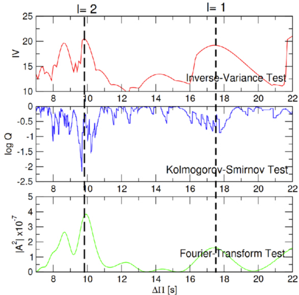
Figure 6. from Ozcan Caliskan et al 2025 Astrophys. J. 988 doi:10.3847/1538-4357/addc70 https://dx.doi.org/10.3847/1538-4357/addc70 © 2025. The Author(s). Published by the American Astronomical Society.
