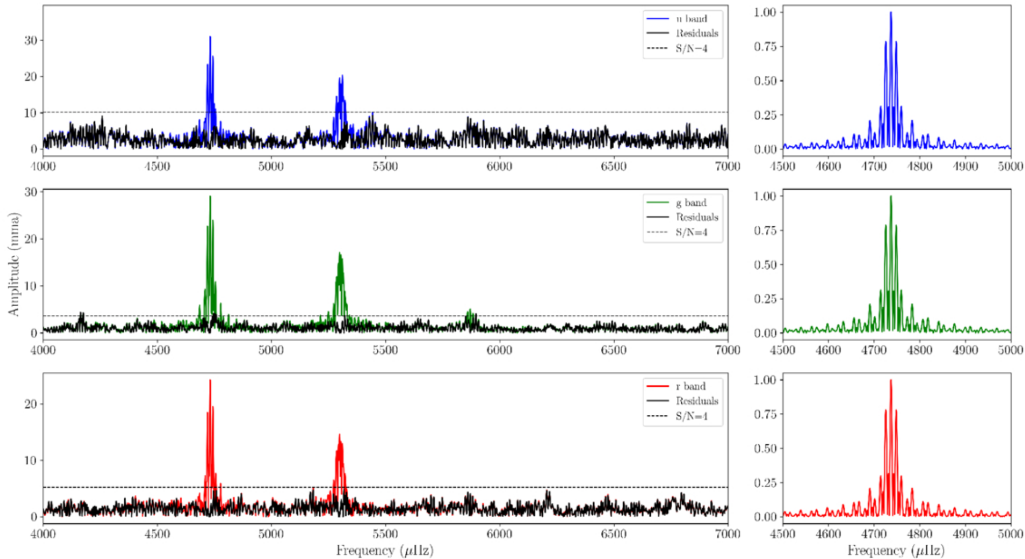
Figure 3. from Ozcan Caliskan et al 2025 Astrophys. J. 988 doi:10.3847/1538-4357/addc70 https://dx.doi.org/10.3847/1538-4357/addc70 © 2025. The Author(s). Published by the American Astronomical Society.
