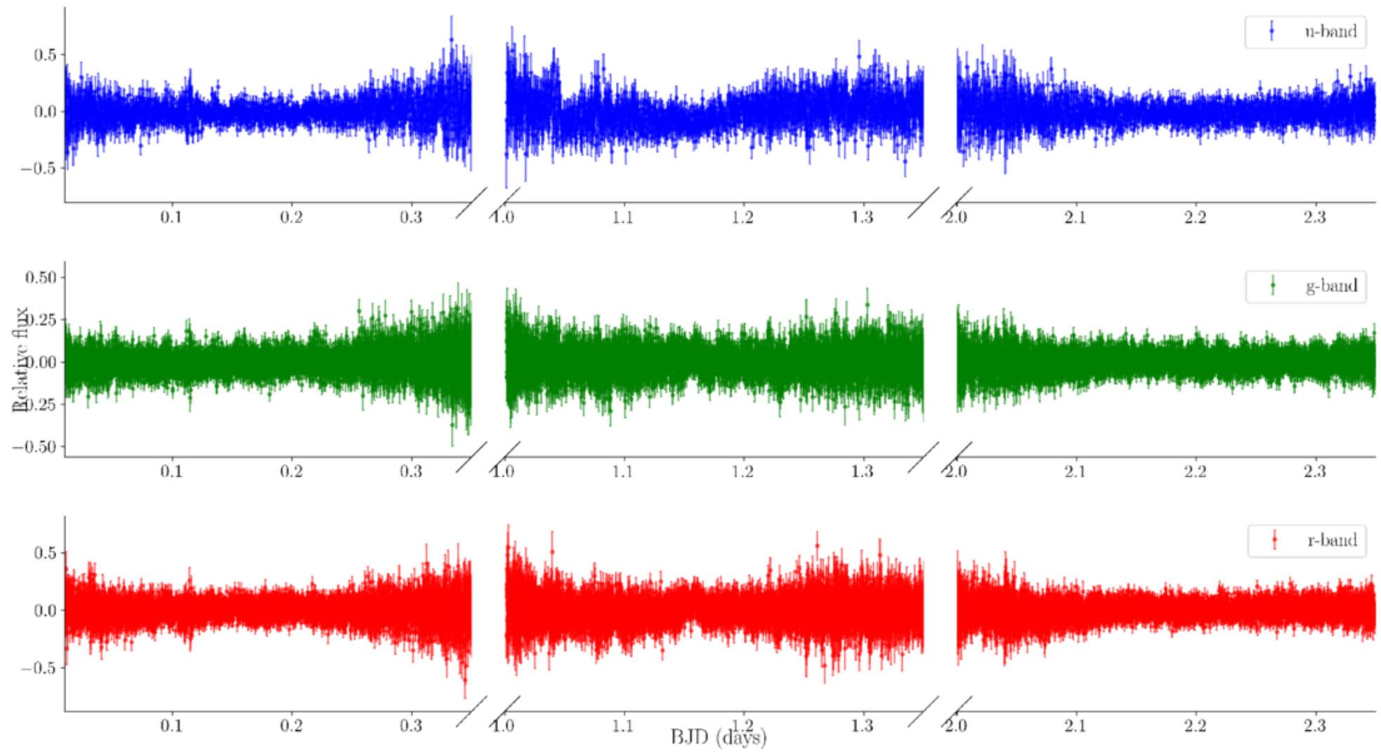
Figure 2. from Ozcan Caliskan et al 2025 Astrophys. J. 988 doi:10.3847/1538-4357/addc70 https://dx.doi.org/10.3847/1538-4357/addc70 © 2025. The Author(s). Published by the American Astronomical Society.
