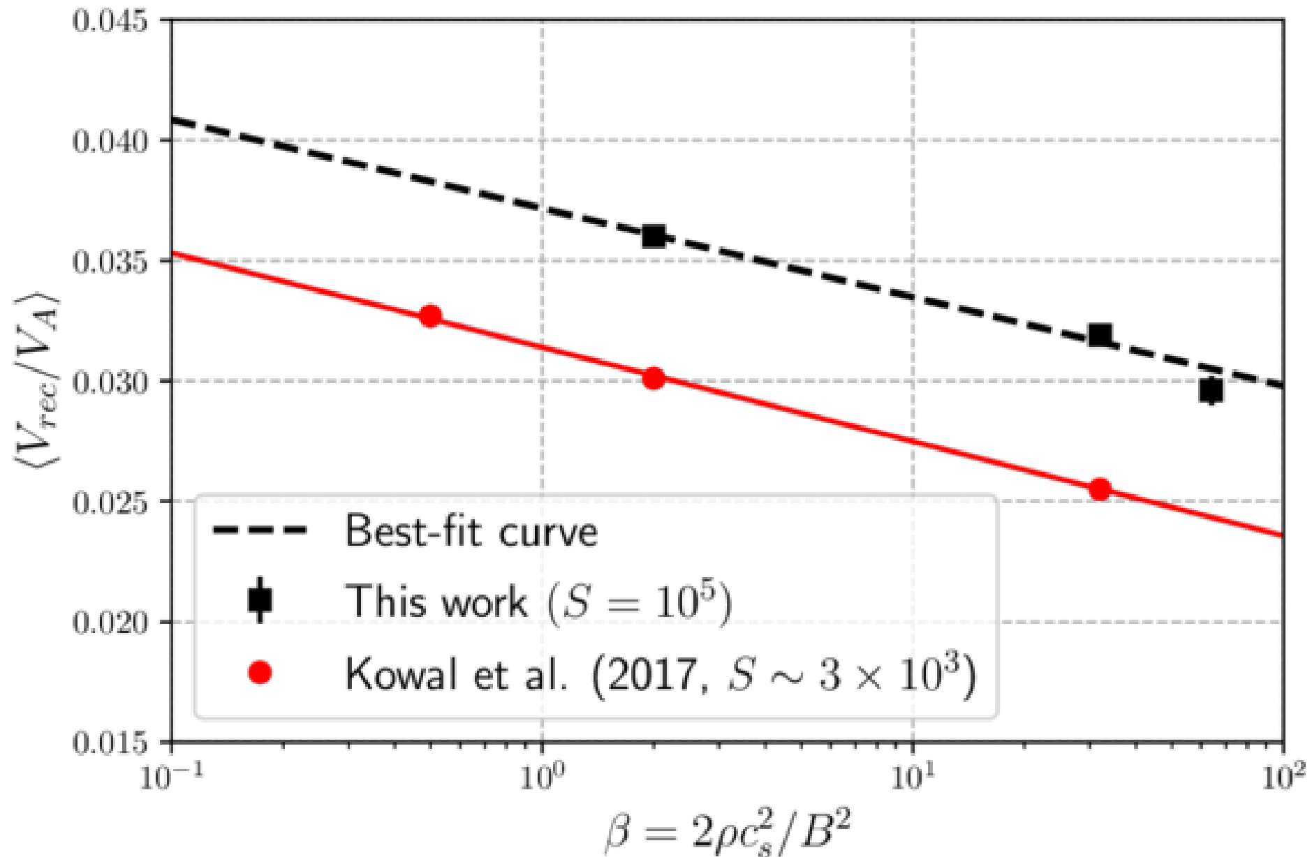
Figure 8. from Giovanni H. Vicentin et al 2025 Astrophys. J. 987 doi:10.3847/1538-4357/addc62 https://dx.doi.org/10.3847/1538-4357/addc62 © 2025. The Author(s). Published by the American Astronomical Society.
