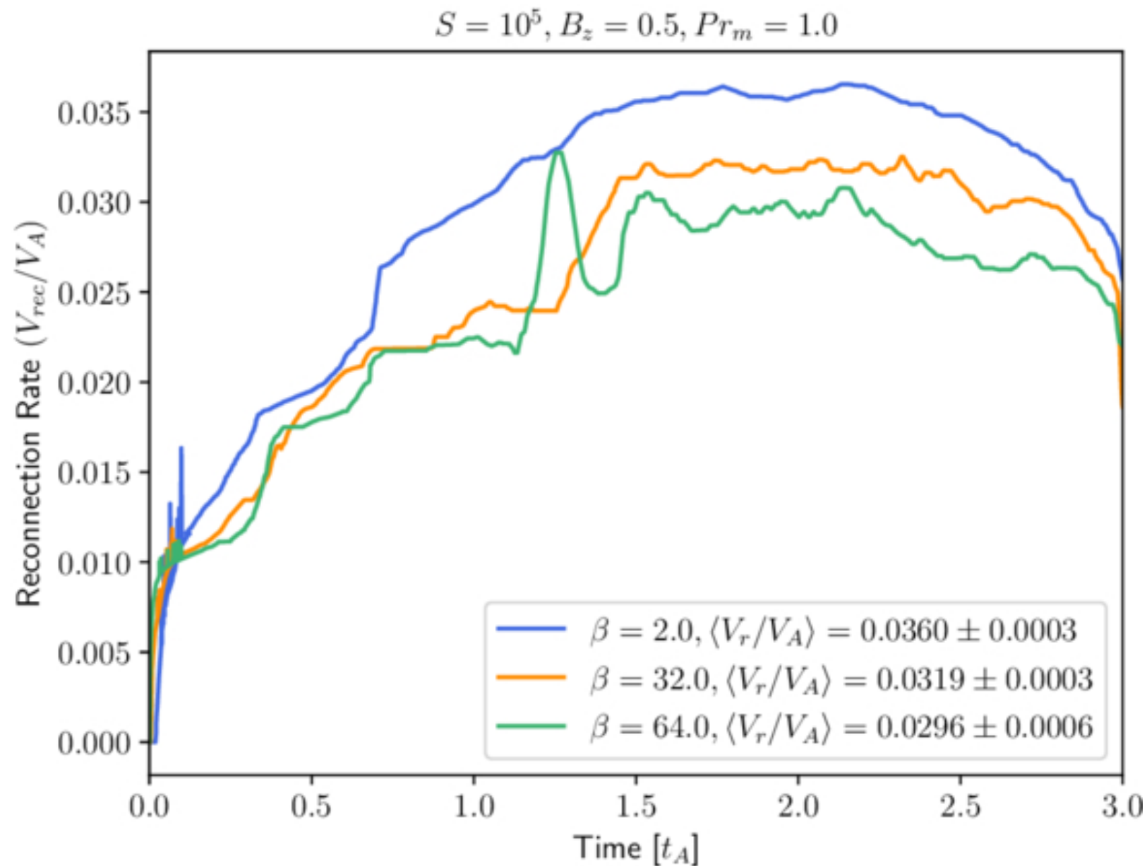
Figure 7. from Giovanni H. Vicentin et al 2025 Astrophys. J. 987 doi:10.3847/1538-4357/addc62 https://dx.doi.org/10.3847/1538-4357/addc62 © 2025. The Author(s). Published by the American Astronomical Society.
