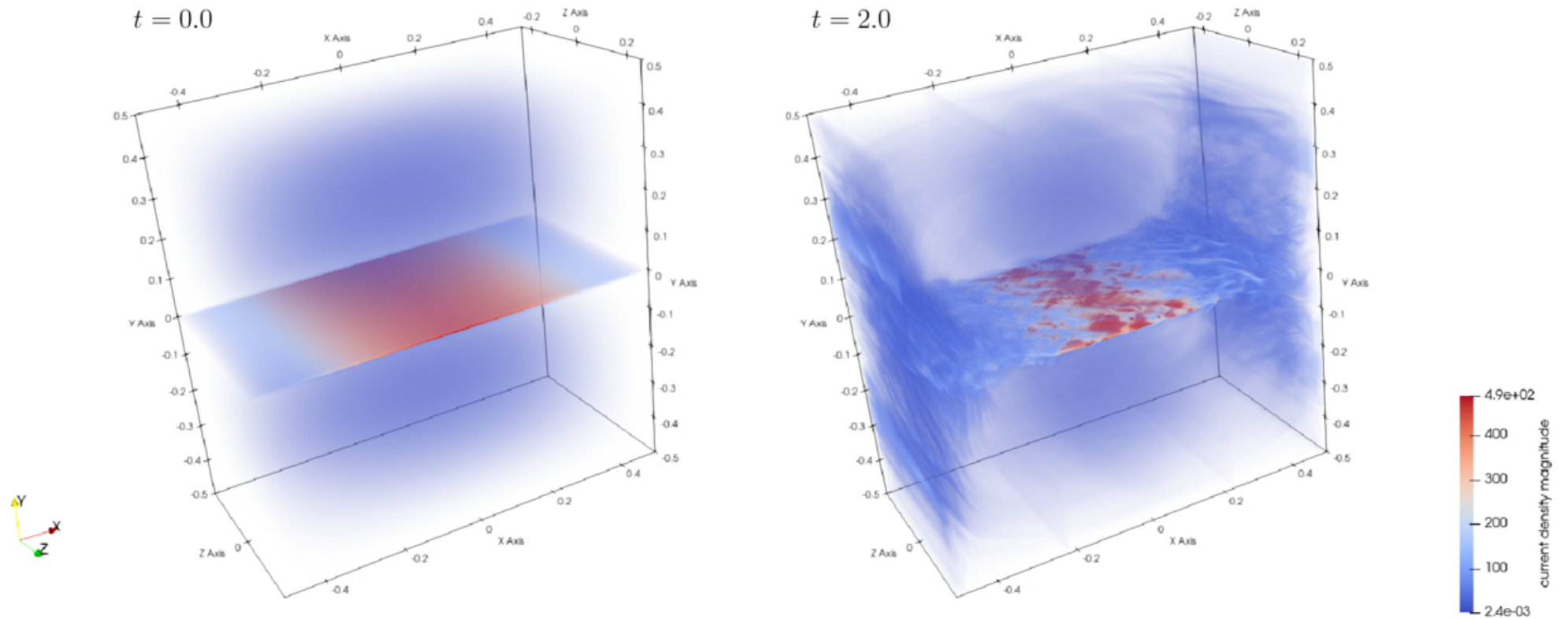
Figure 3. from Giovanni H. Vicentin et al 2025 Astrophys. J. 987 doi:10.3847/1538-4357/addc62 https://dx.doi.org/10.3847/1538-4357/addc62 © 2025. The Author(s). Published by the American Astronomical Society.
