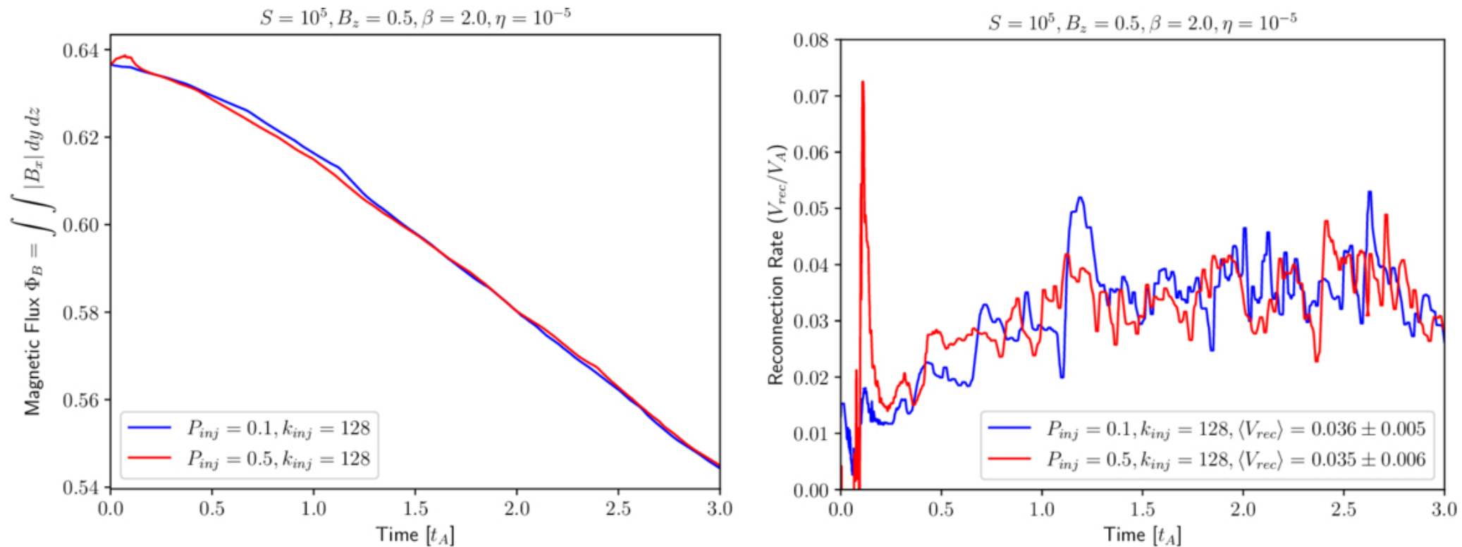
Figure 21. from Giovanni H. Vicentin et al 2025 Astrophys. J. 987 doi:10.3847/1538-4357/addc62 https://dx.doi.org/10.3847/1538-4357/addc62 © 2025. The Author(s). Published by the American Astronomical Society.
