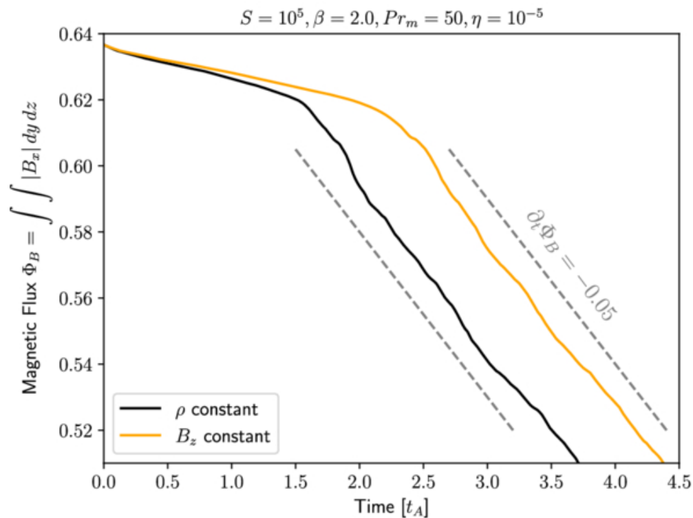
Figure 20. from Giovanni H. Vicentin et al 2025 Astrophys. J. 987 doi:10.3847/1538-4357/addc62 https://dx.doi.org/10.3847/1538-4357/addc62 © 2025. The Author(s). Published by the American Astronomical Society.
