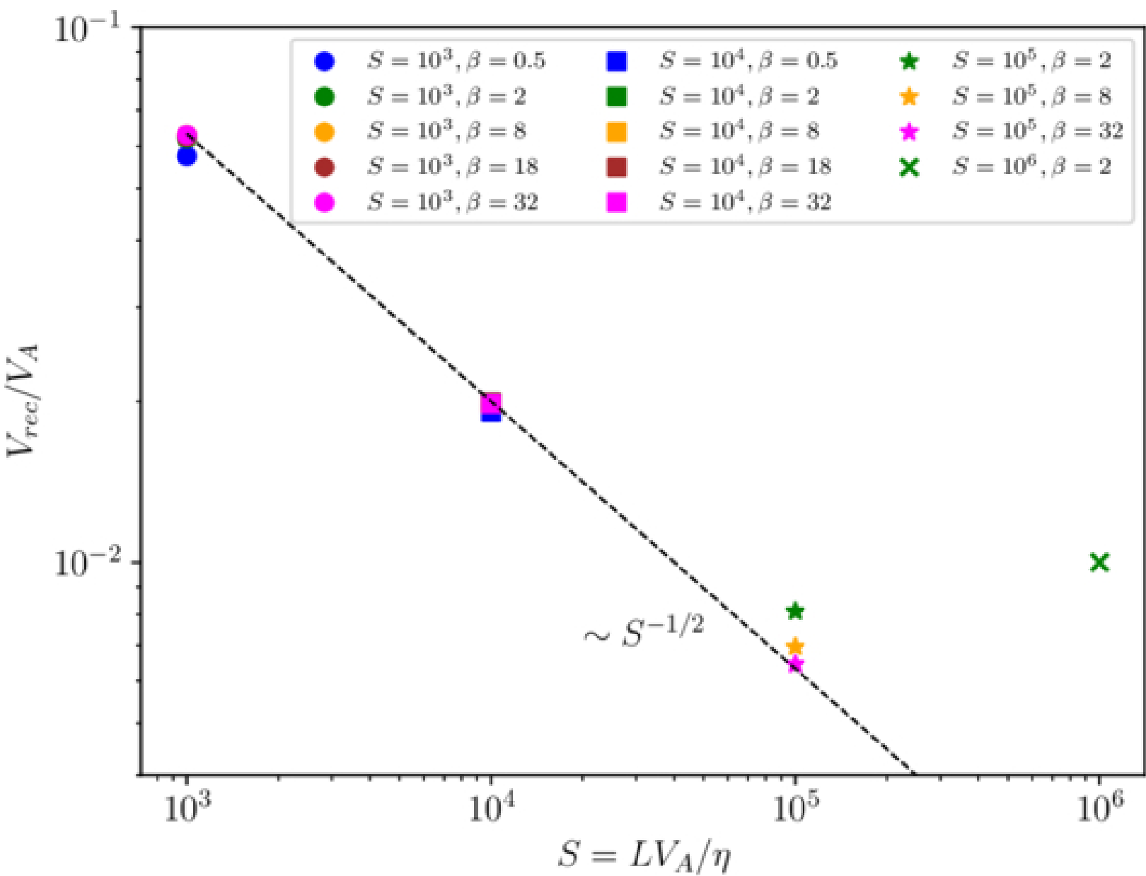
Figure 2. from Giovanni H. Vicentin et al 2025 Astrophys. J. 987 doi:10.3847/1538-4357/addc62 https://dx.doi.org/10.3847/1538-4357/addc62 © 2025. The Author(s). Published by the American Astronomical Society.
