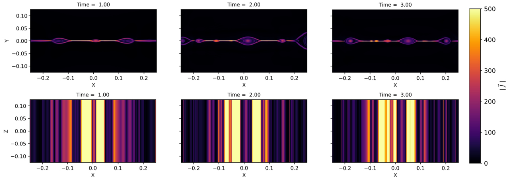
Figure 16. from Giovanni H. Vicentin et al 2025 Astrophys. J. 987 doi:10.3847/1538-4357/addc62 https://dx.doi.org/10.3847/1538-4357/addc62 © 2025. The Author(s). Published by the American Astronomical Society.
