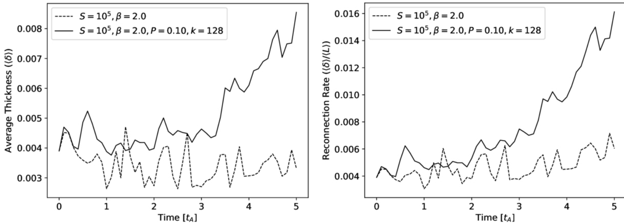
Figure 15. from Giovanni H. Vicentin et al 2025 Astrophys. J. 987 doi:10.3847/1538-4357/addc62 https://dx.doi.org/10.3847/1538-4357/addc62 © 2025. The Author(s). Published by the American Astronomical Society.
