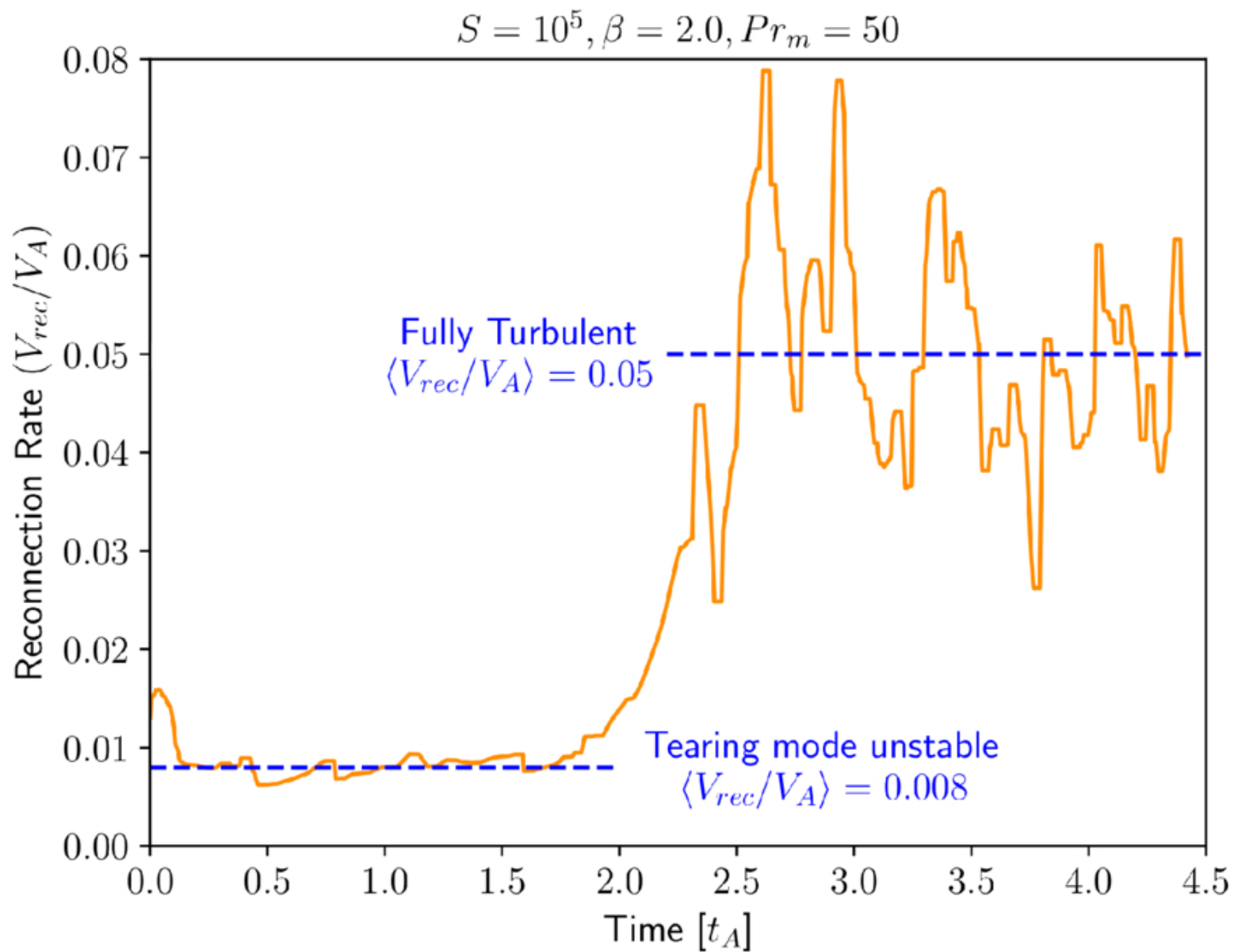
Figure 13. from Giovanni H. Vicentin et al 2025 Astrophys. J. 987 doi:10.3847/1538-4357/addc62 https://dx.doi.org/10.3847/1538-4357/addc62 © 2025. The Author(s). Published by the American Astronomical Society.
