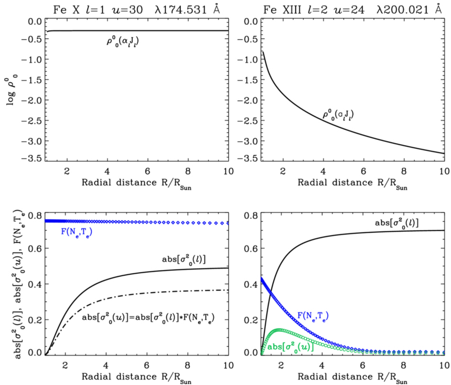
Figure 7. from Nataliia G. Shchukina et al 2025 Astrophys. J. 988 doi:10.3847/1538-4357/addc61 https://dx.doi.org/10.3847/1538-4357/addc61 © 2025. The Author(s). Published by the American Astronomical Society.
