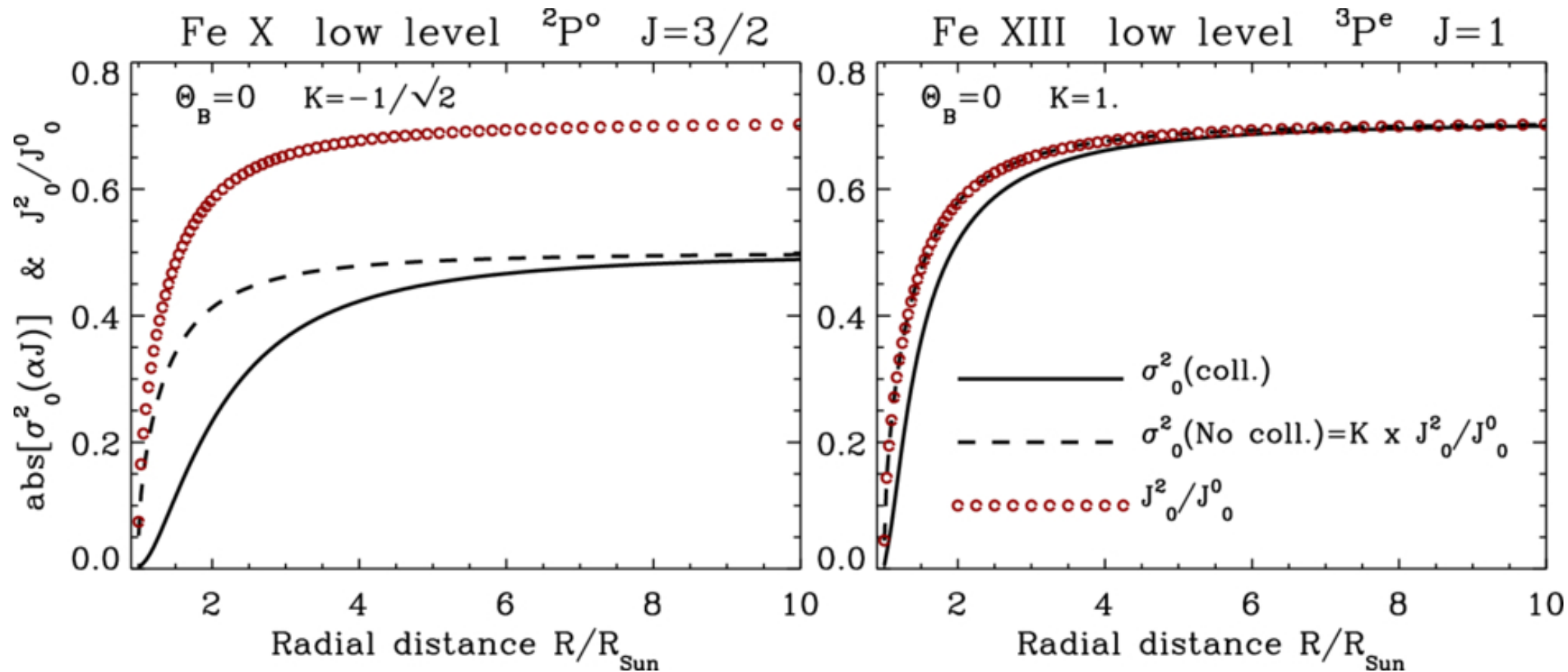
Figure 6. from Nataliia G. Shchukina et al 2025 Astrophys. J. 988 doi:10.3847/1538-4357/addc61 https://dx.doi.org/10.3847/1538-4357/addc61 © 2025. The Author(s). Published by the American Astronomical Society.
