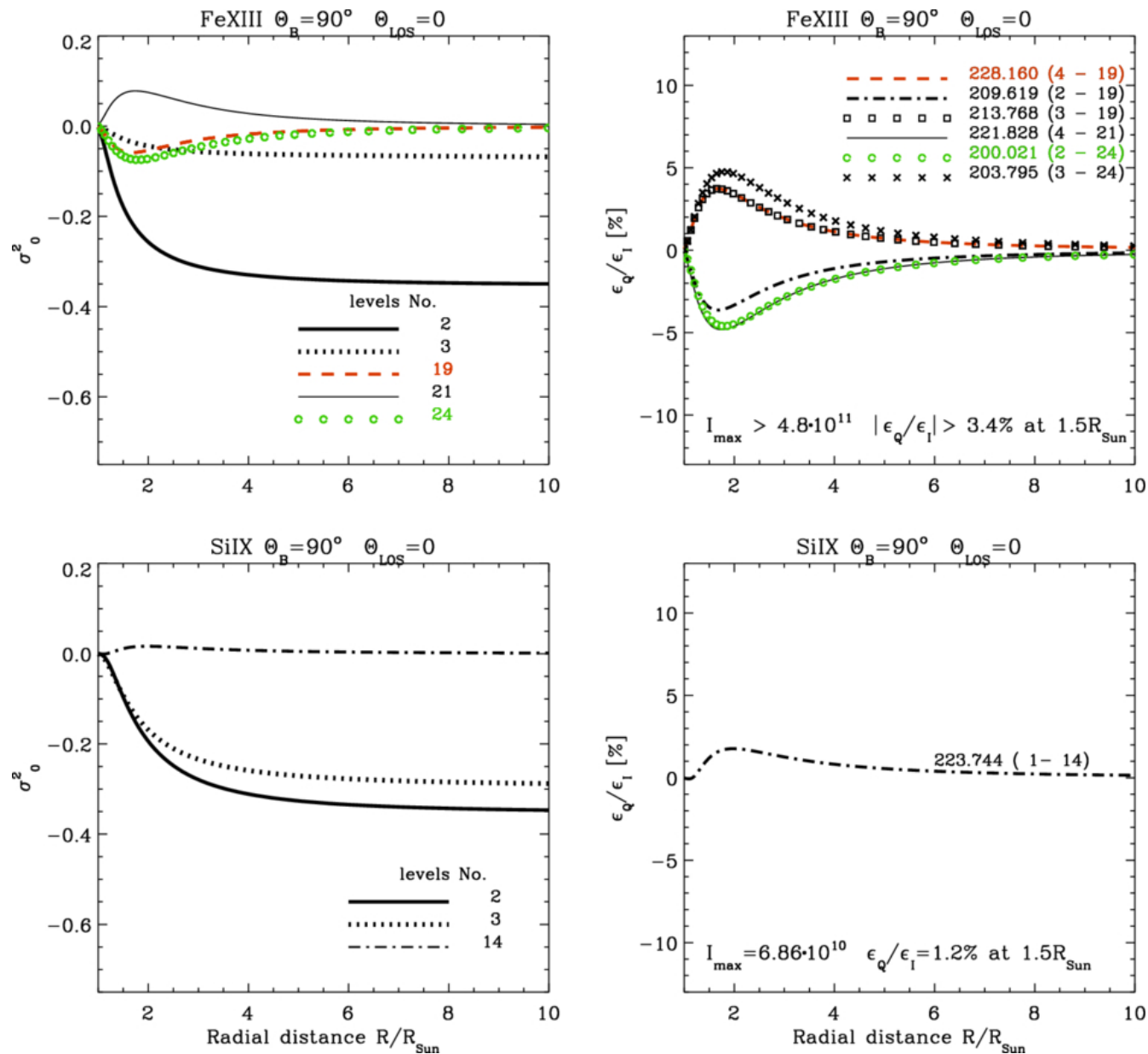
Figure 5. from Nataliia G. Shchukina et al 2025 Astrophys. J. 988 doi:10.3847/1538-4357/addc61 https://dx.doi.org/10.3847/1538-4357/addc61 © 2025. The Author(s). Published by the American Astronomical Society.
