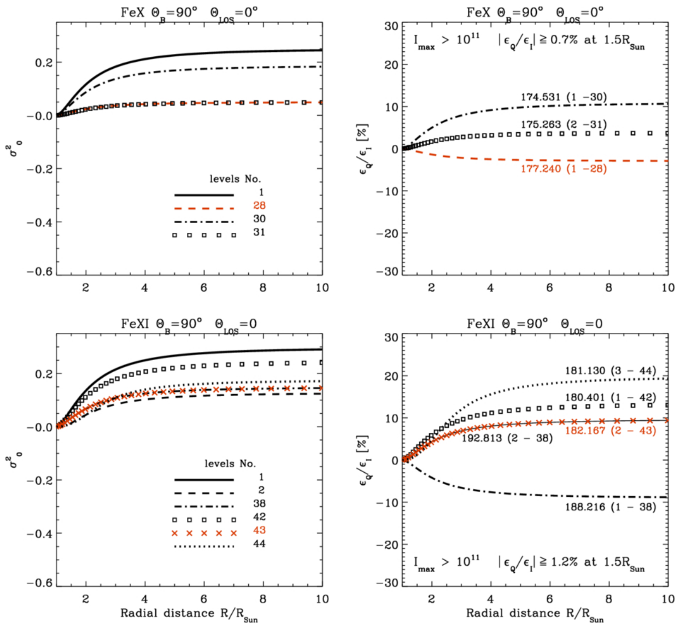
Figure 4. from Nataliia G. Shchukina et al 2025 Astrophys. J. 988 doi:10.3847/1538-4357/addc61 https://dx.doi.org/10.3847/1538-4357/addc61 © 2025. The Author(s). Published by the American Astronomical Society.
