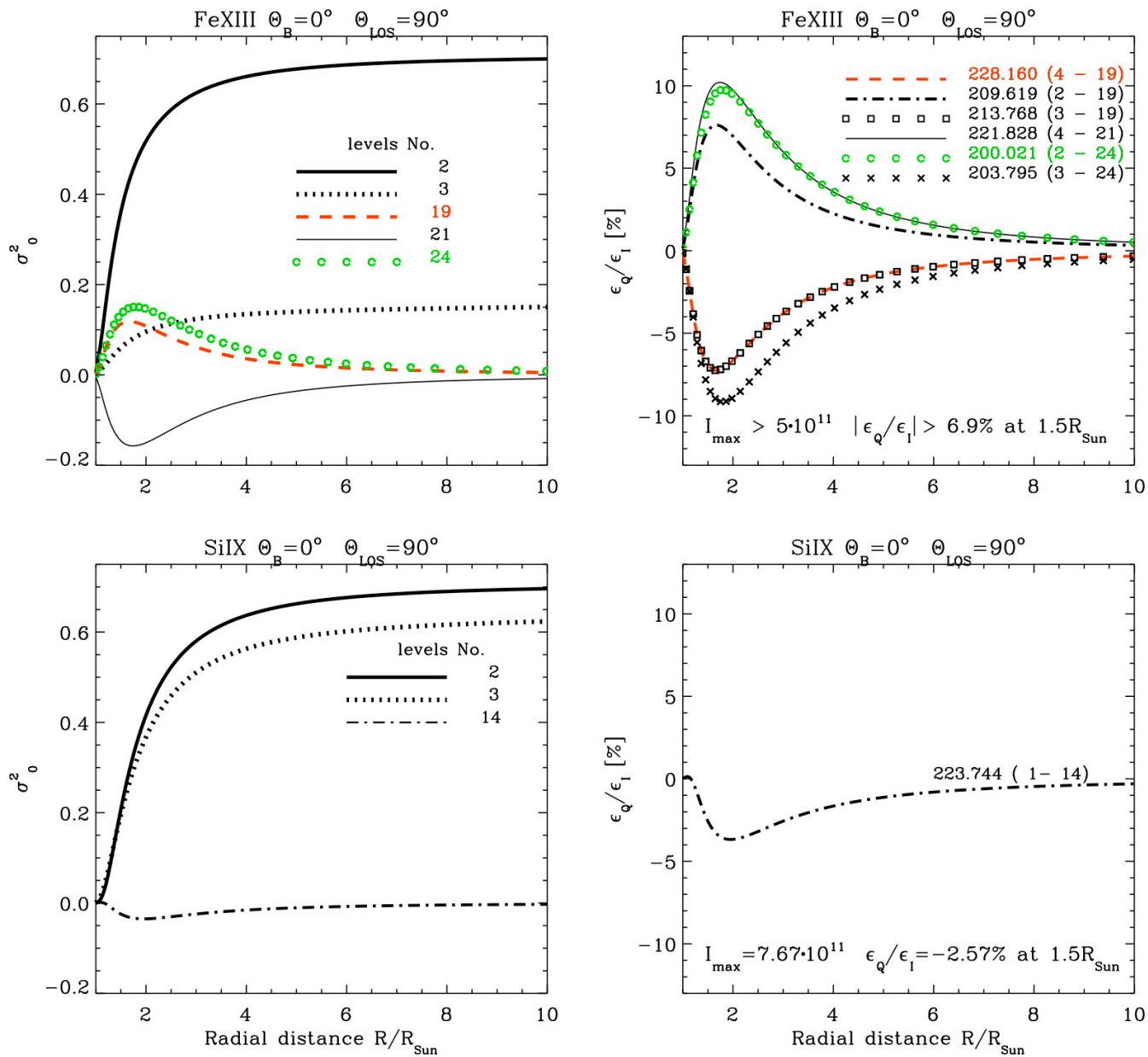
Figure 3. from Nataliia G. Shchukina et al 2025 Astrophys. J. 988 doi:10.3847/1538-4357/addc61 https://dx.doi.org/10.3847/1538-4357/addc61 © 2025. The Author(s). Published by the American Astronomical Society.
