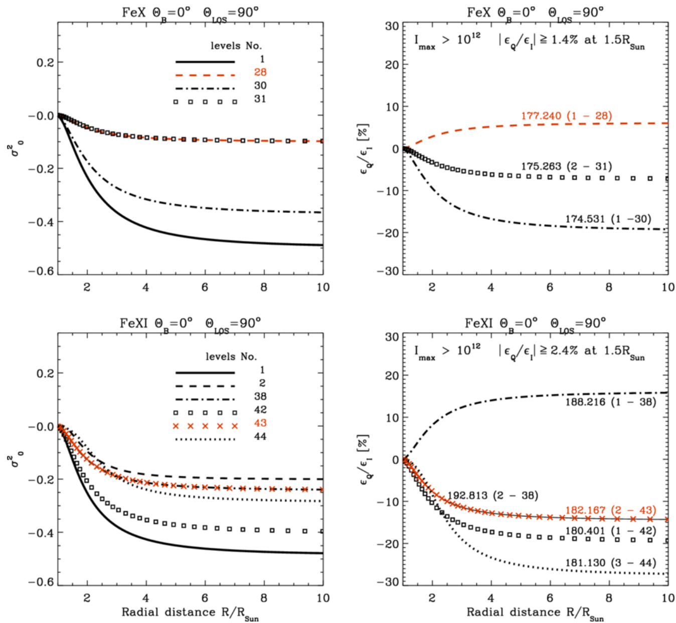
Figure 2. from Nataliia G. Shchukina et al 2025 Astrophys. J. 988 doi:10.3847/1538-4357/addc61 https://dx.doi.org/10.3847/1538-4357/addc61 © 2025. The Author(s). Published by the American Astronomical Society.
