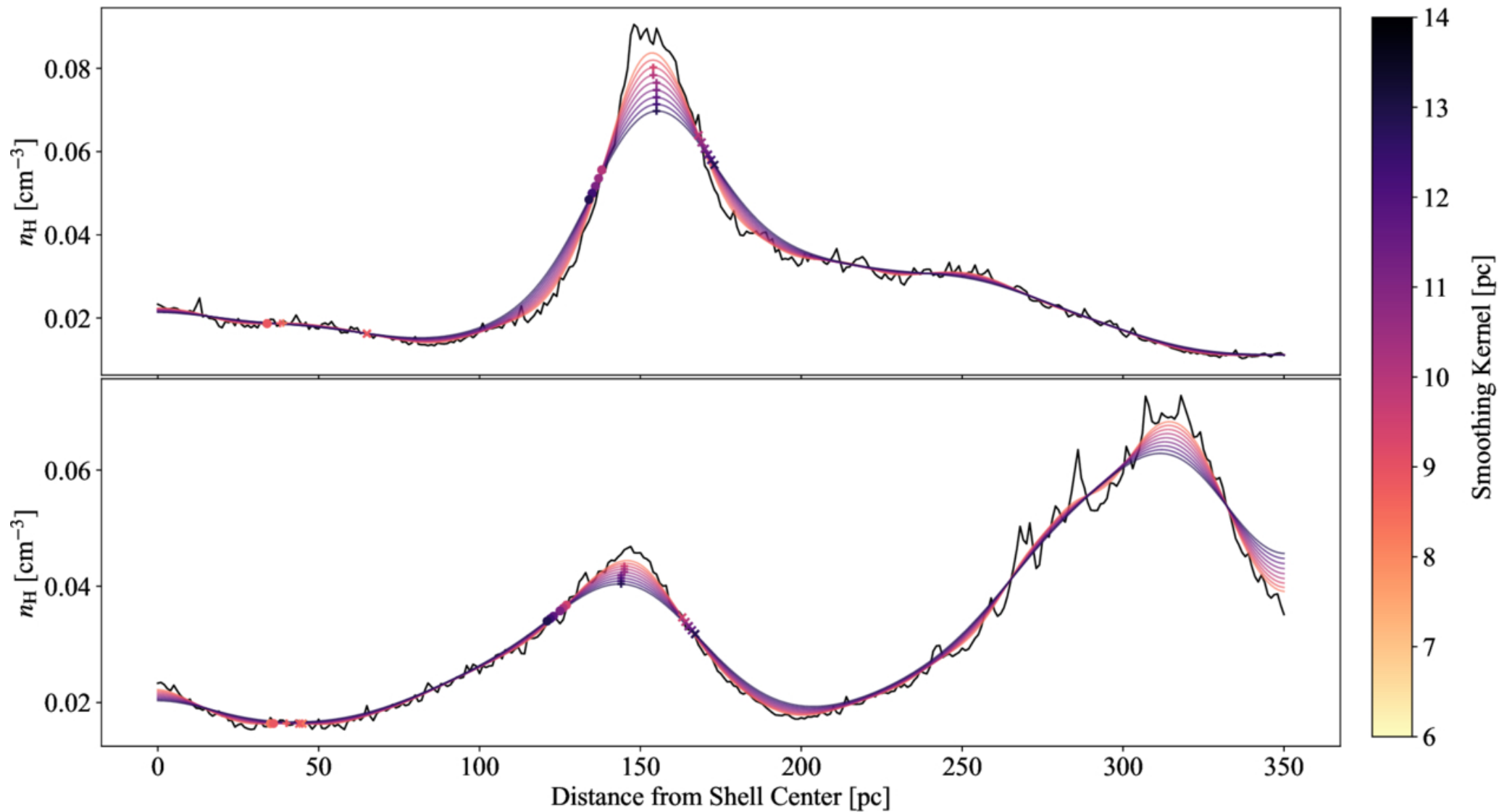
Figure 9. from Bore Annie Gao et al 2025 Astrophys. J. 987 doi:10.3847/1538-4357/add7d8 https://dx.doi.org/10.3847/1538-4357/add7d8 © 2025. The Author(s). Published by the American Astronomical Society.
