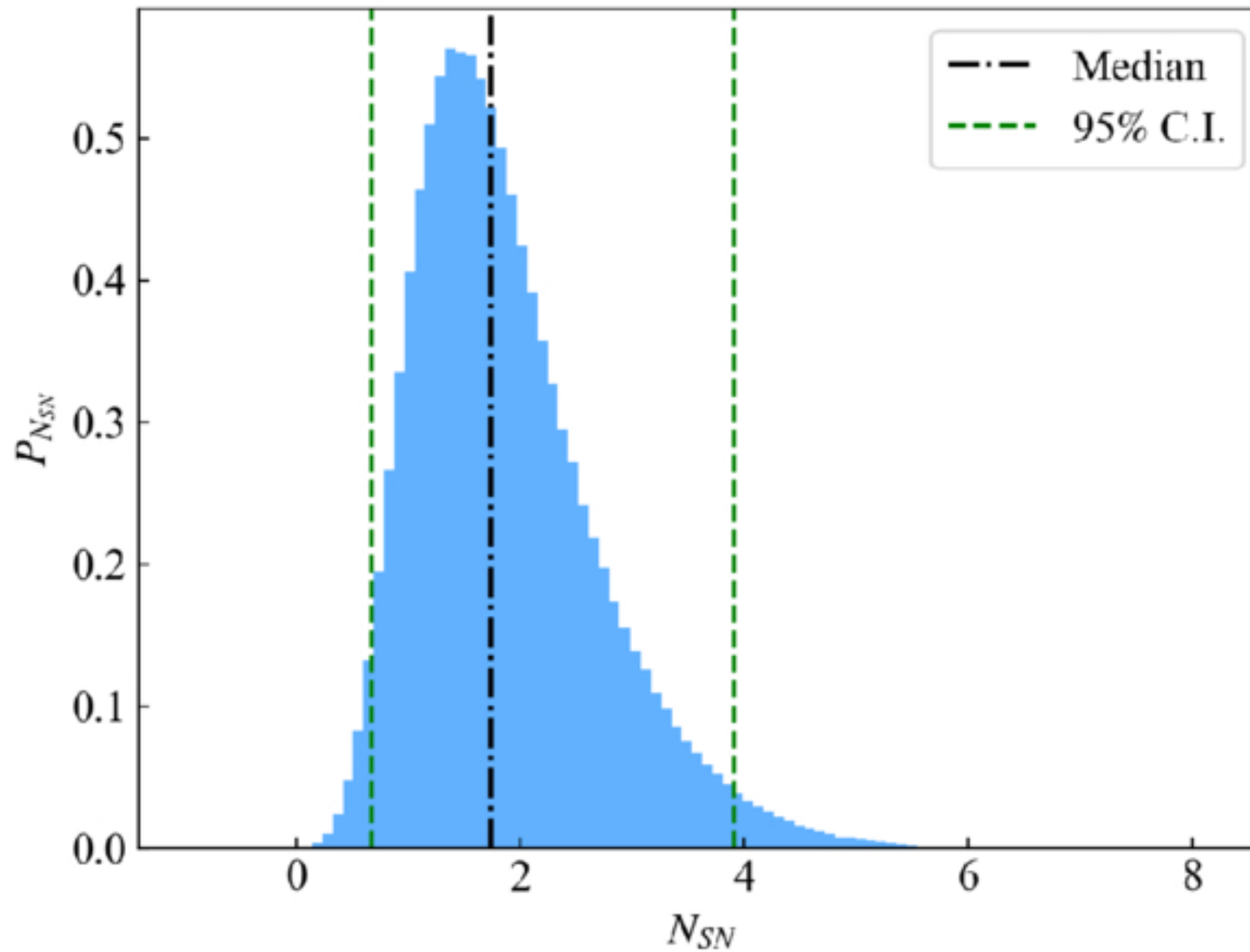
Figure 7. from Bore Annie Gao et al 2025 Astrophys. J. 987 doi:10.3847/1538-4357/add7d8 https://dx.doi.org/10.3847/1538-4357/add7d8 © 2025. The Author(s). Published by the American Astronomical Society.
