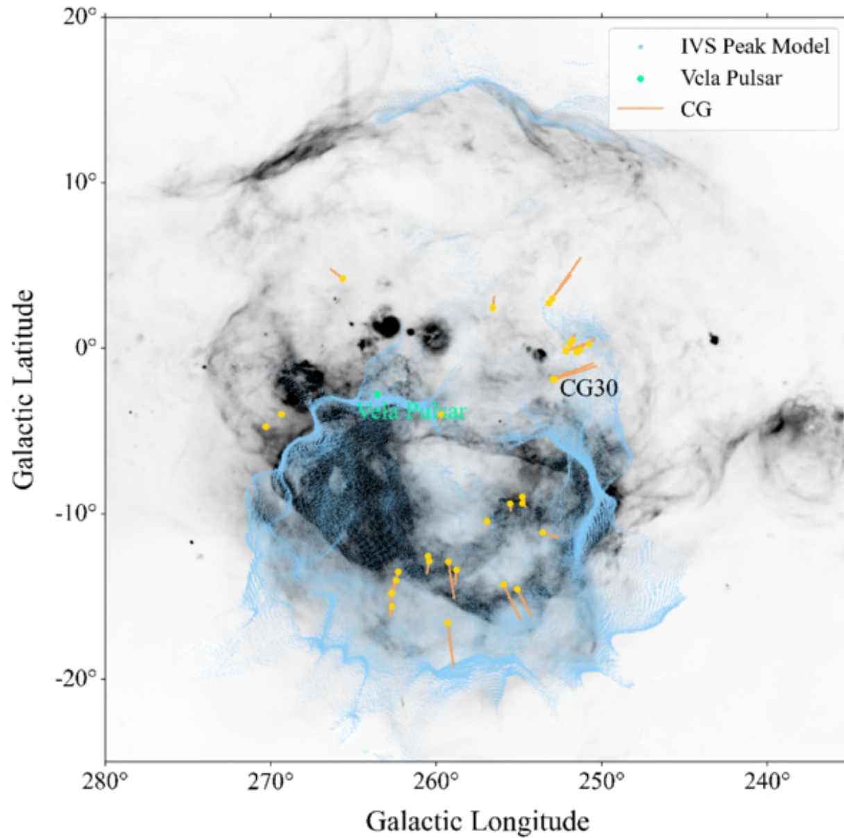
Figure 6. from Bore Annie Gao et al 2025 Astrophys. J. 987 doi:10.3847/1538-4357/add7d8 https://dx.doi.org/10.3847/1538-4357/add7d8 © 2025. The Author(s). Published by the American Astronomical Society.
