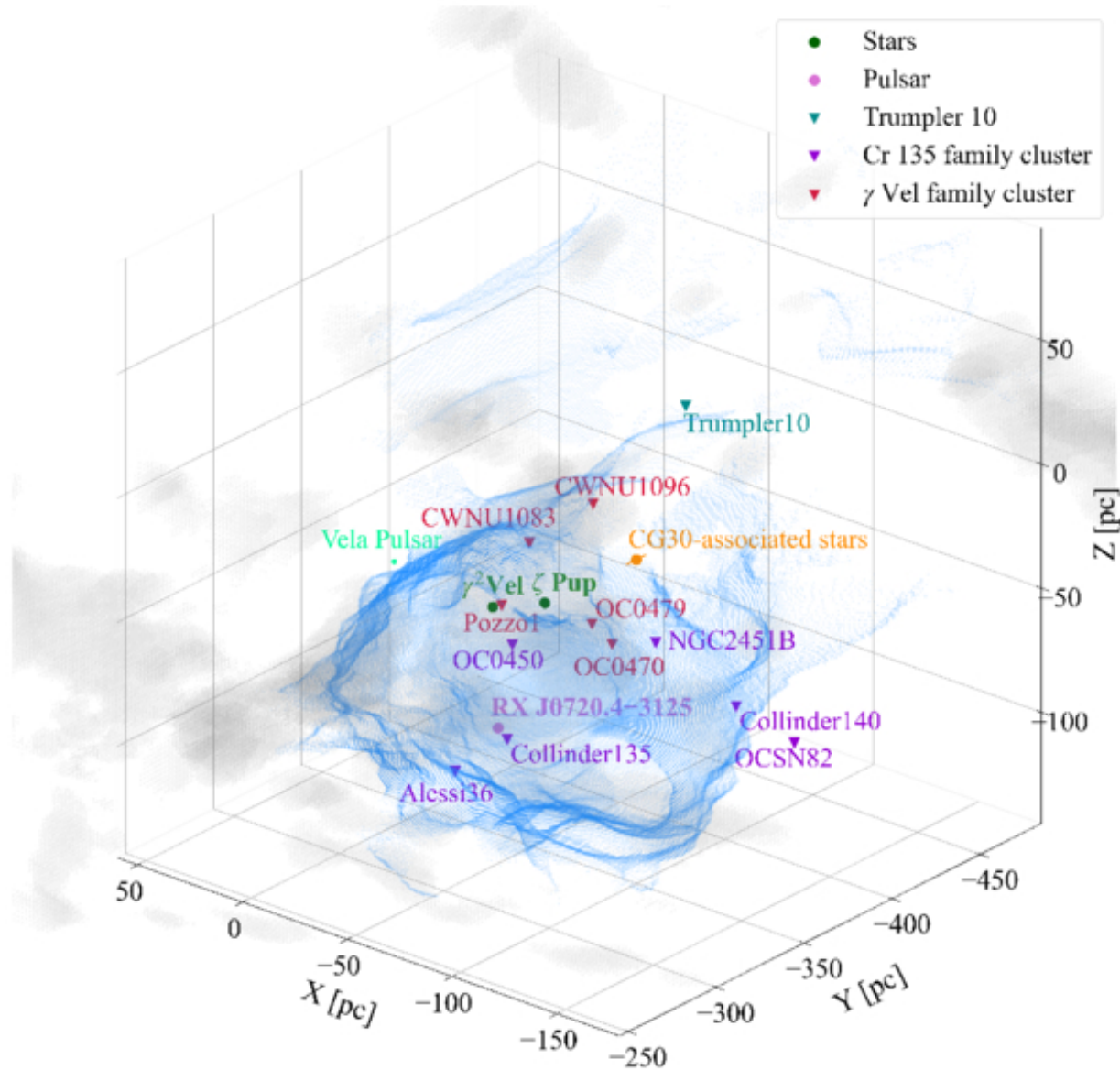
Figure 5. from Bore Annie Gao et al 2025 Astrophys. J. 987 doi:10.3847/1538-4357/add7d8 https://dx.doi.org/10.3847/1538-4357/add7d8 © 2025. The Author(s). Published by the American Astronomical Society.
