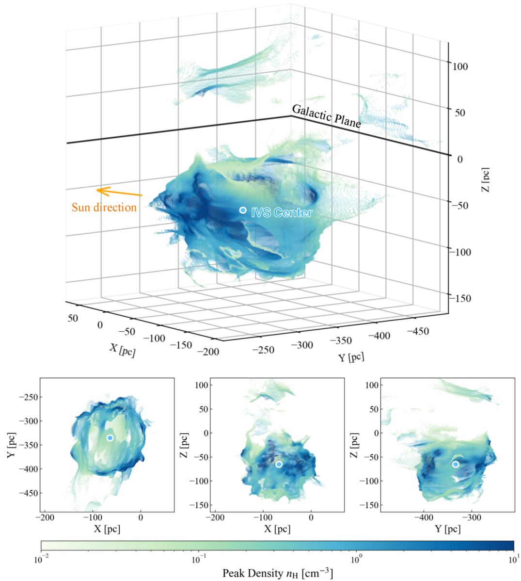
Figure 3. from Bore Annie Gao et al 2025 Astrophys. J. 987 doi:10.3847/1538-4357/add7d8 https://dx.doi.org/10.3847/1538-4357/add7d8 © 2025. The Author(s). Published by the American Astronomical Society.
