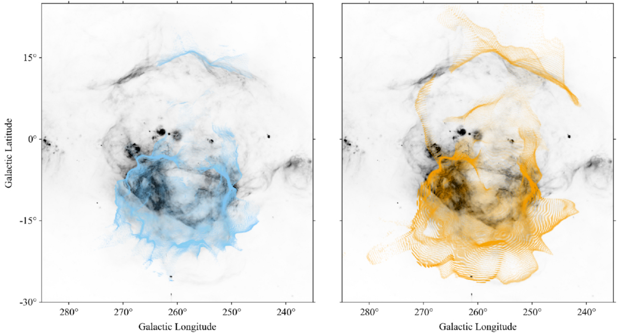
Figure 10. from Bore Annie Gao et al 2025 Astrophys. J. 987 doi:10.3847/1538-4357/add7d8 https://dx.doi.org/10.3847/1538-4357/add7d8 © 2025. The Author(s). Published by the American Astronomical Society.
