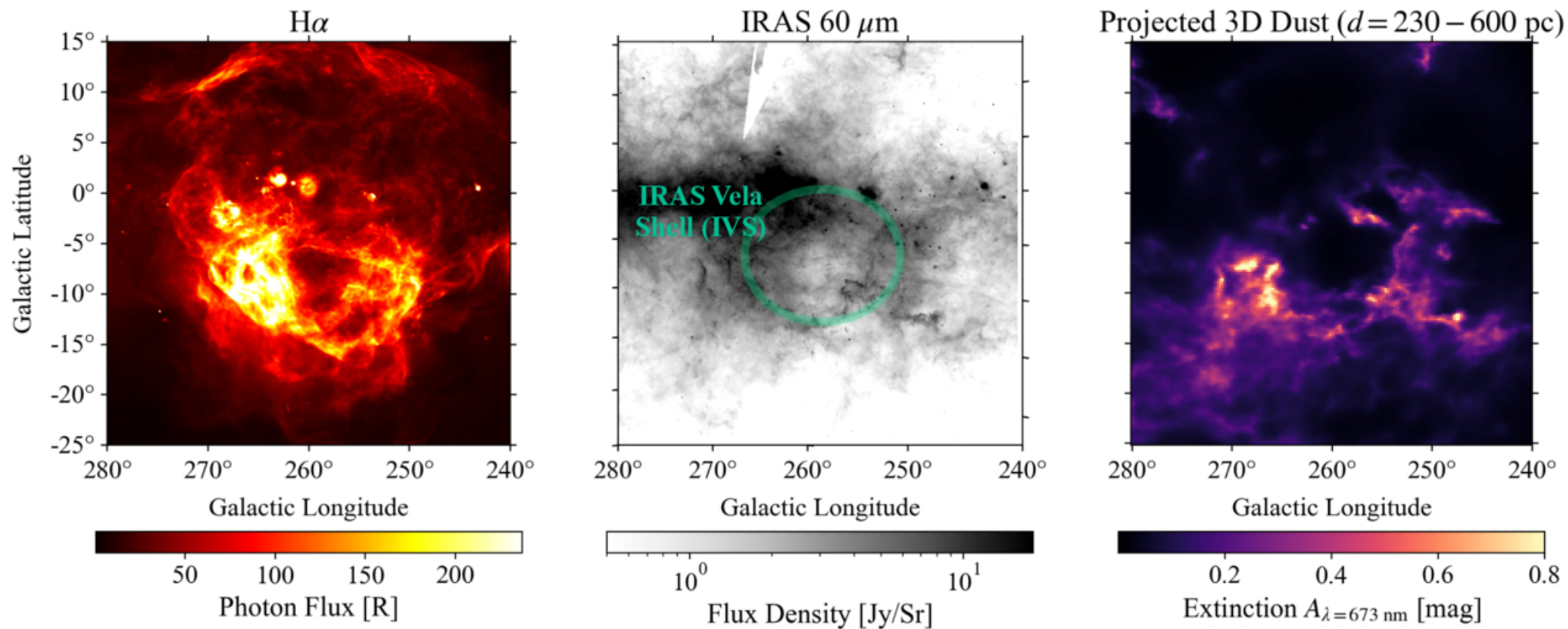
Figure 1. from Bore Annie Gao et al 2025 Astrophys. J. 987 doi:10.3847/1538-4357/add7d8 https://dx.doi.org/10.3847/1538-4357/add7d8 © 2025. The Author(s). Published by the American Astronomical Society.
