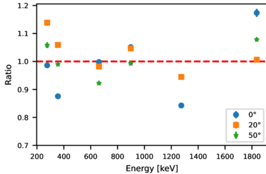
Figure 8. from Savitri Gallego et al 2025 Astrophys. J. 986 doi:10.3847/1538-4357/add6a0 https://dx.doi.org/10.3847/1538-4357/add6a0 © 2025. The Author(s). Published by the American Astronomical Society.
