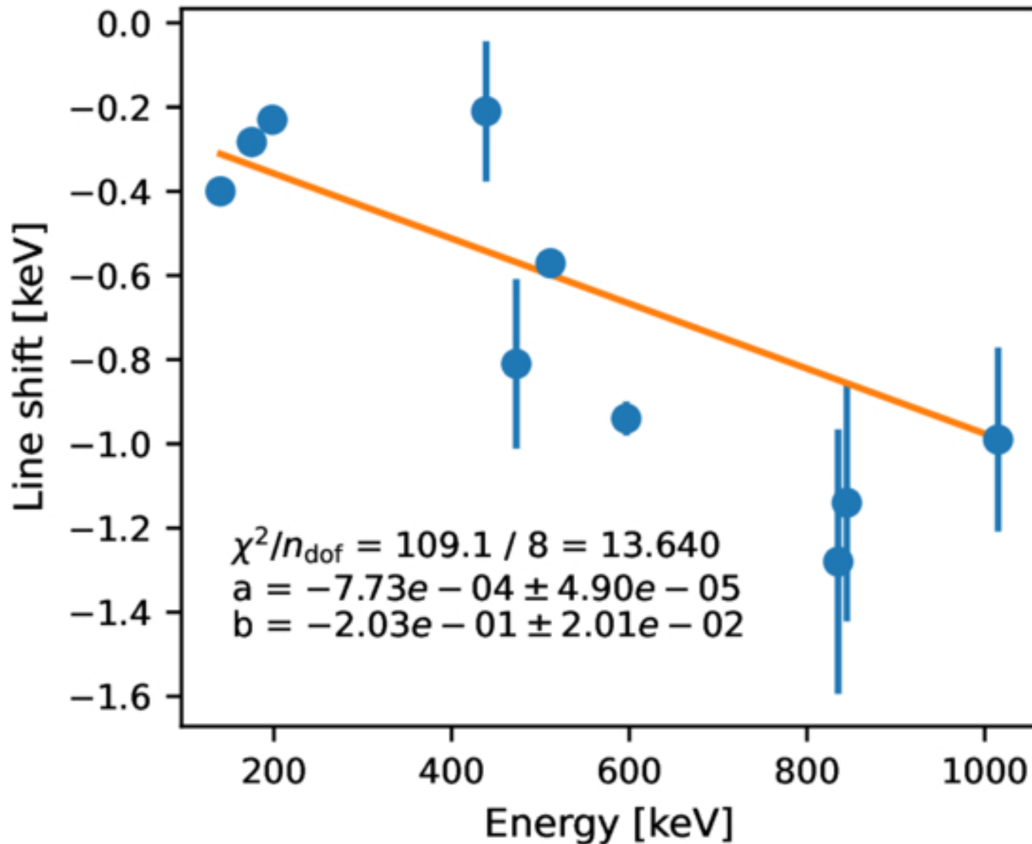
Figure 7. from Savitri Gallego et al 2025 Astrophys. J. 986 doi:10.3847/1538-4357/add6a0 https://dx.doi.org/10.3847/1538-4357/add6a0 © 2025. The Author(s). Published by the American Astronomical Society.
