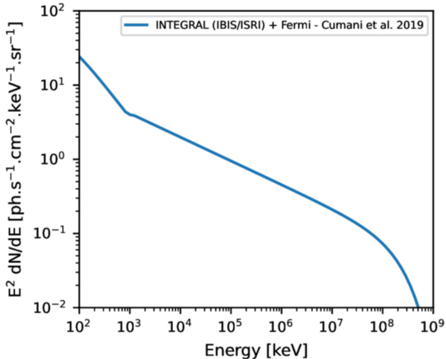
Figure 5. from Savitri Gallego et al 2025 Astrophys. J. 986 doi:10.3847/1538-4357/add6a0 https://dx.doi.org/10.3847/1538-4357/add6a0 © 2025. The Author(s). Published by the American Astronomical Society.
