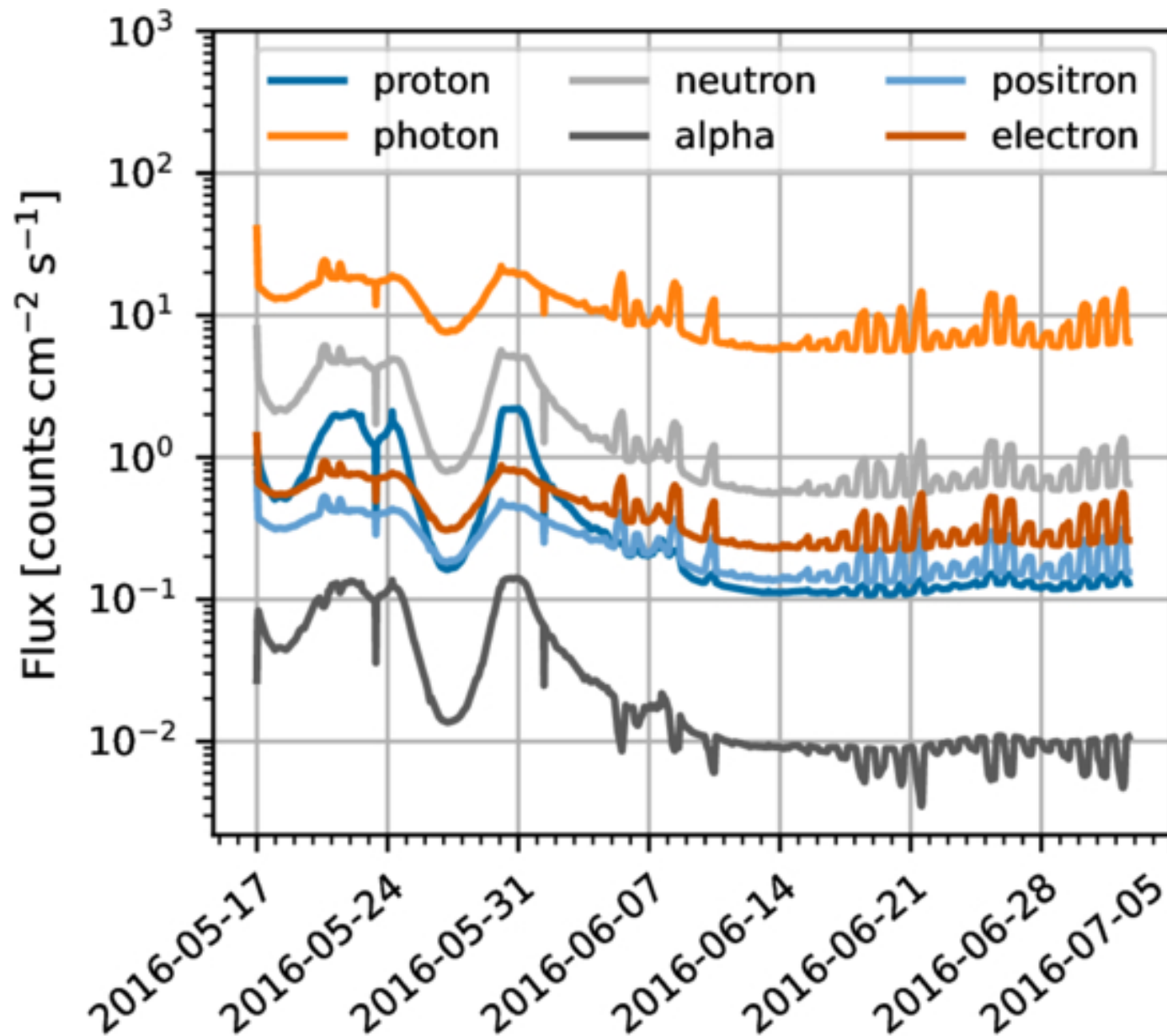
Figure 4. from Savitri Gallego et al 2025 Astrophys. J. 986 doi:10.3847/1538-4357/add6a0 https://dx.doi.org/10.3847/1538-4357/add6a0 © 2025. The Author(s). Published by the American Astronomical Society.
