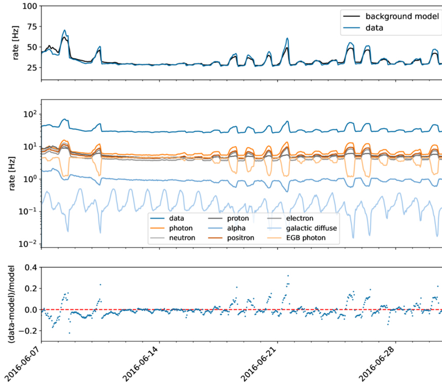
Figure 14. from Savitri Gallego et al 2025 Astrophys. J. 986 doi:10.3847/1538-4357/add6a0 https://dx.doi.org/10.3847/1538-4357/add6a0 © 2025. The Author(s). Published by the American Astronomical Society.
