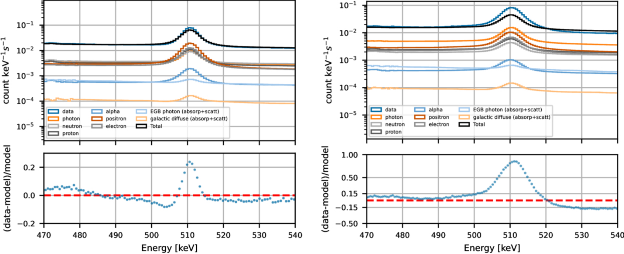
Figure 13. from Savitri Gallego et al 2025 Astrophys. J. 986 doi:10.3847/1538-4357/add6a0 https://dx.doi.org/10.3847/1538-4357/add6a0 © 2025. The Author(s). Published by the American Astronomical Society.
