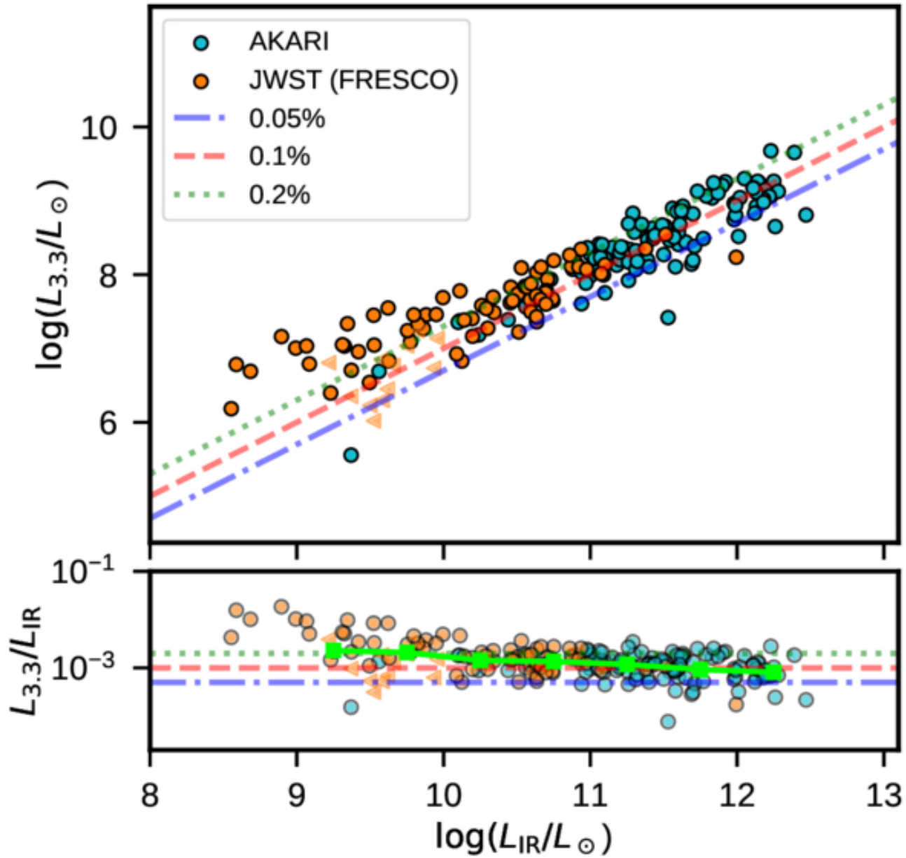
Figure 3. from Jianwei Lyu et al 2025 Astrophys. J. 986 doi:10.3847/1538-4357/add538 https://dx.doi.org/10.3847/1538-4357/add538 © 2025. The Author(s). Published by the American Astronomical Society.
