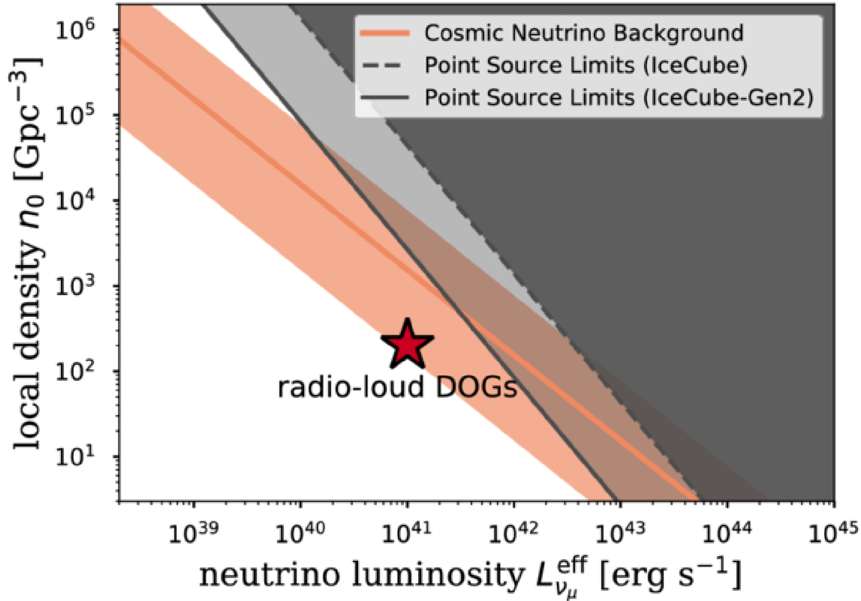
Figure 6. from Hikaru Fukuchi et al 2025 Astrophys. J. 987 doi:10.3847/1538-4357/add478 https://dx.doi.org/10.3847/1538-4357/add478 © 2025. The Author(s). Published by the American Astronomical Society.
