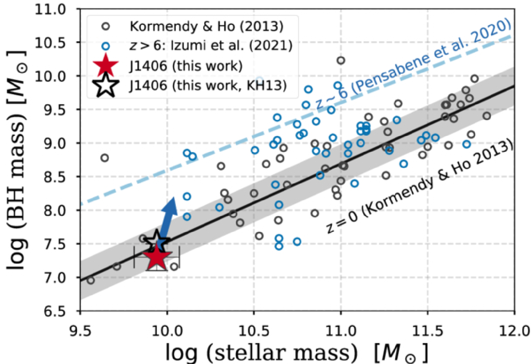
Figure 5. from Hikaru Fukuchi et al 2025 Astrophys. J. 987 doi:10.3847/1538-4357/add478 https://dx.doi.org/10.3847/1538-4357/add478 © 2025. The Author(s). Published by the American Astronomical Society.
