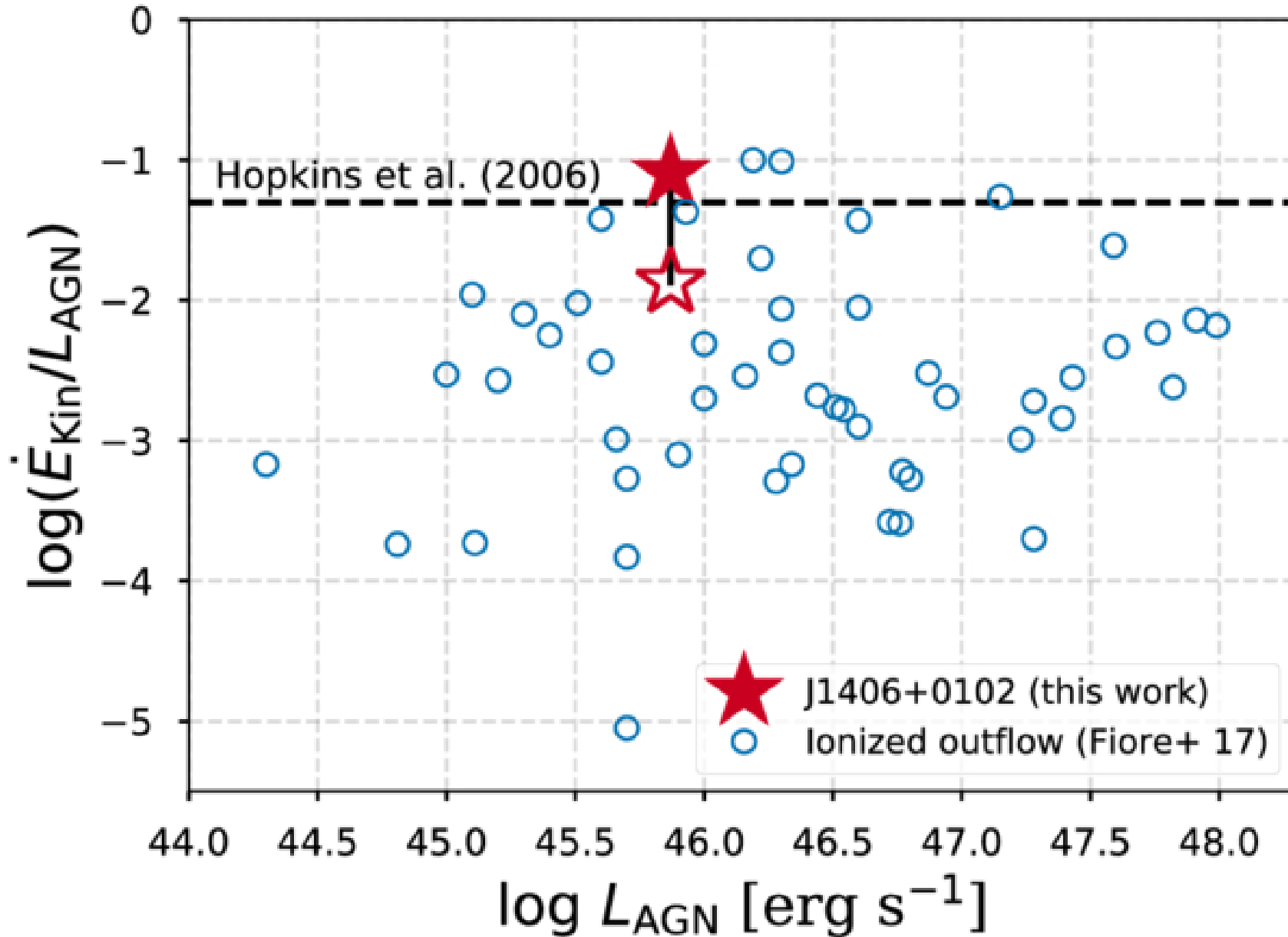
Figure 4. from Hikaru Fukuchi et al 2025 Astrophys. J. 987 doi:10.3847/1538-4357/add478 https://dx.doi.org/10.3847/1538-4357/add478 © 2025. The Author(s). Published by the American Astronomical Society.
