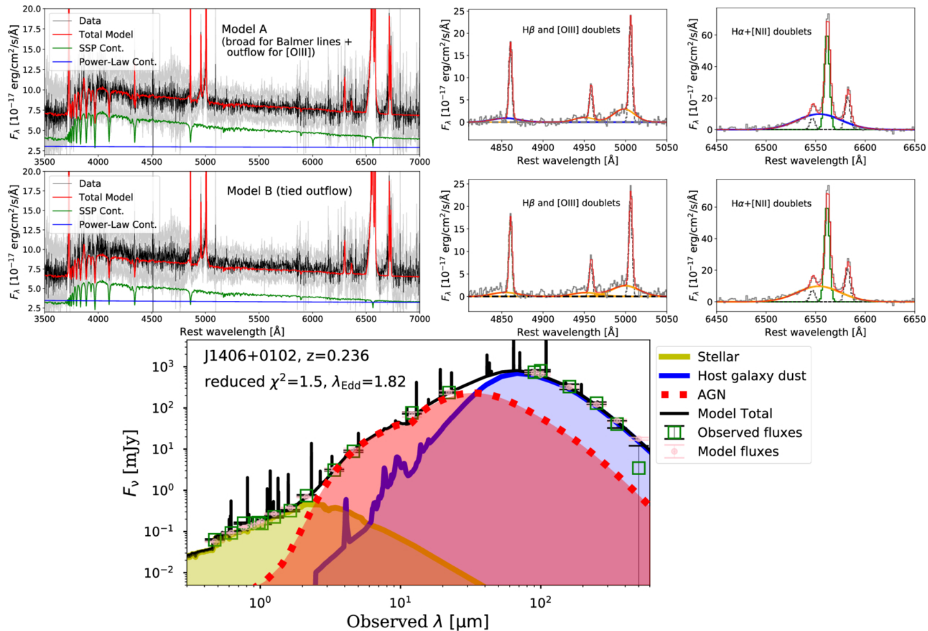
Figure 2. from Hikaru Fukuchi et al 2025 Astrophys. J. 987 doi:10.3847/1538-4357/add478 https://dx.doi.org/10.3847/1538-4357/add478 © 2025. The Author(s). Published by the American Astronomical Society.
