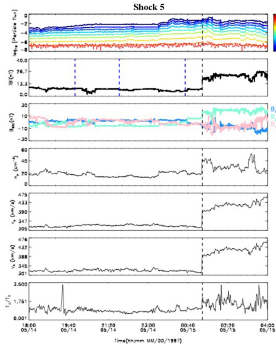
Figure 9. from Shanwlee Sow Mondal et al 2025 Astrophys. J. 987 doi:10.3847/1538-4357/add3f0 https://dx.doi.org/10.3847/1538-4357/add3f0 © 2025. The Author(s). Published by the American Astronomical Society.
