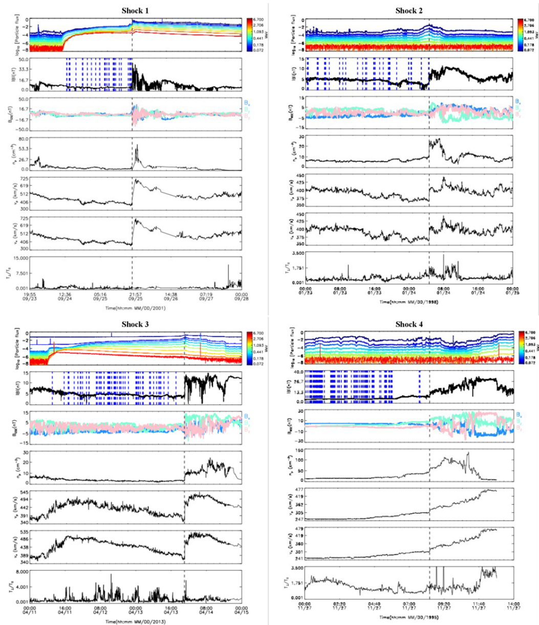
Figure 9. from Shanwlee Sow Mondal et al 2025 Astrophys. J. 987 doi:10.3847/1538-4357/add3f0 https://dx.doi.org/10.3847/1538-4357/add3f0 © 2025. The Author(s). Published by the American Astronomical Society.
