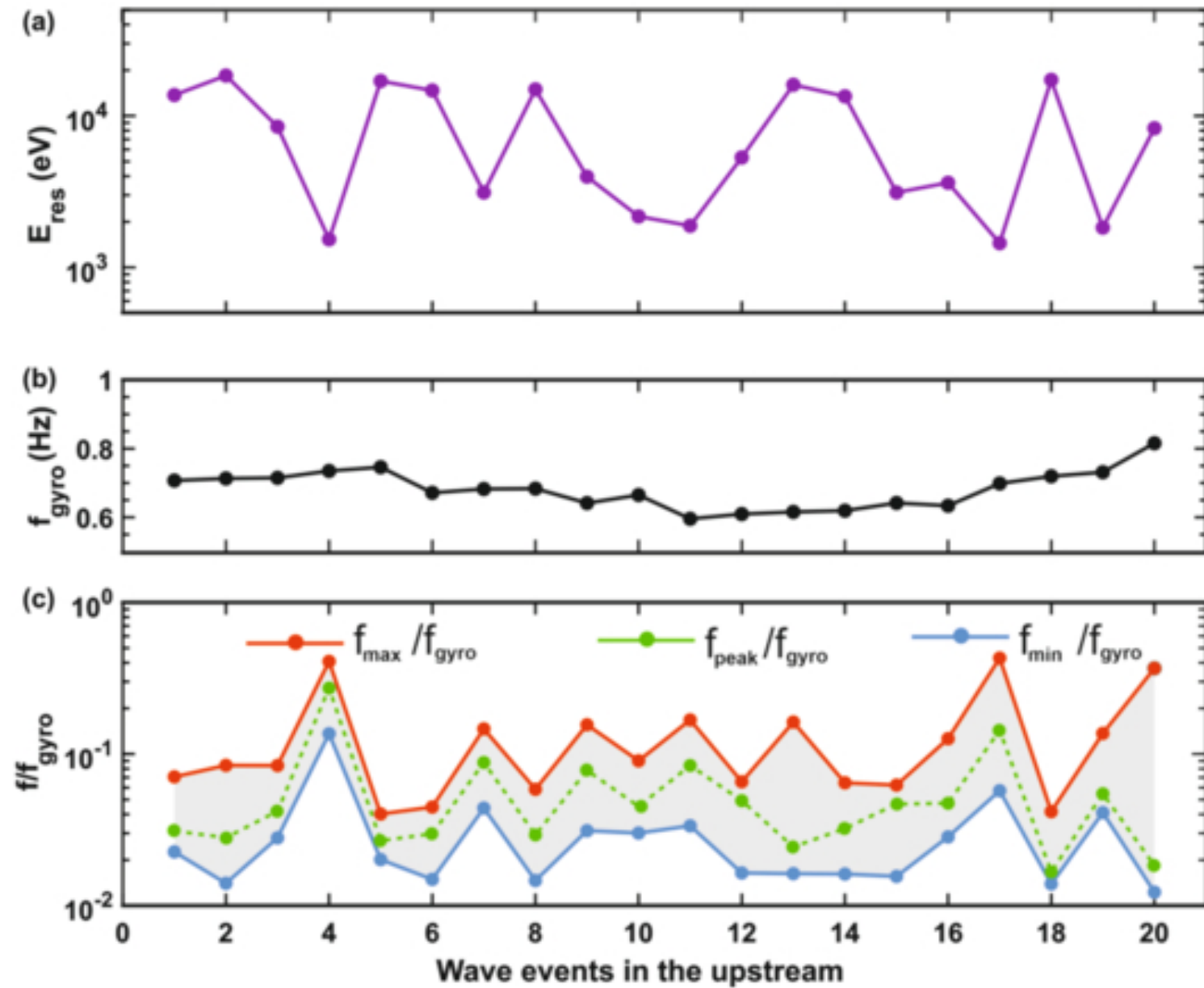
Figure 5. from Shanwlee Sow Mondal et al 2025 Astrophys. J. 987 doi:10.3847/1538-4357/add3f0 https://dx.doi.org/10.3847/1538-4357/add3f0 © 2025. The Author(s). Published by the American Astronomical Society.
