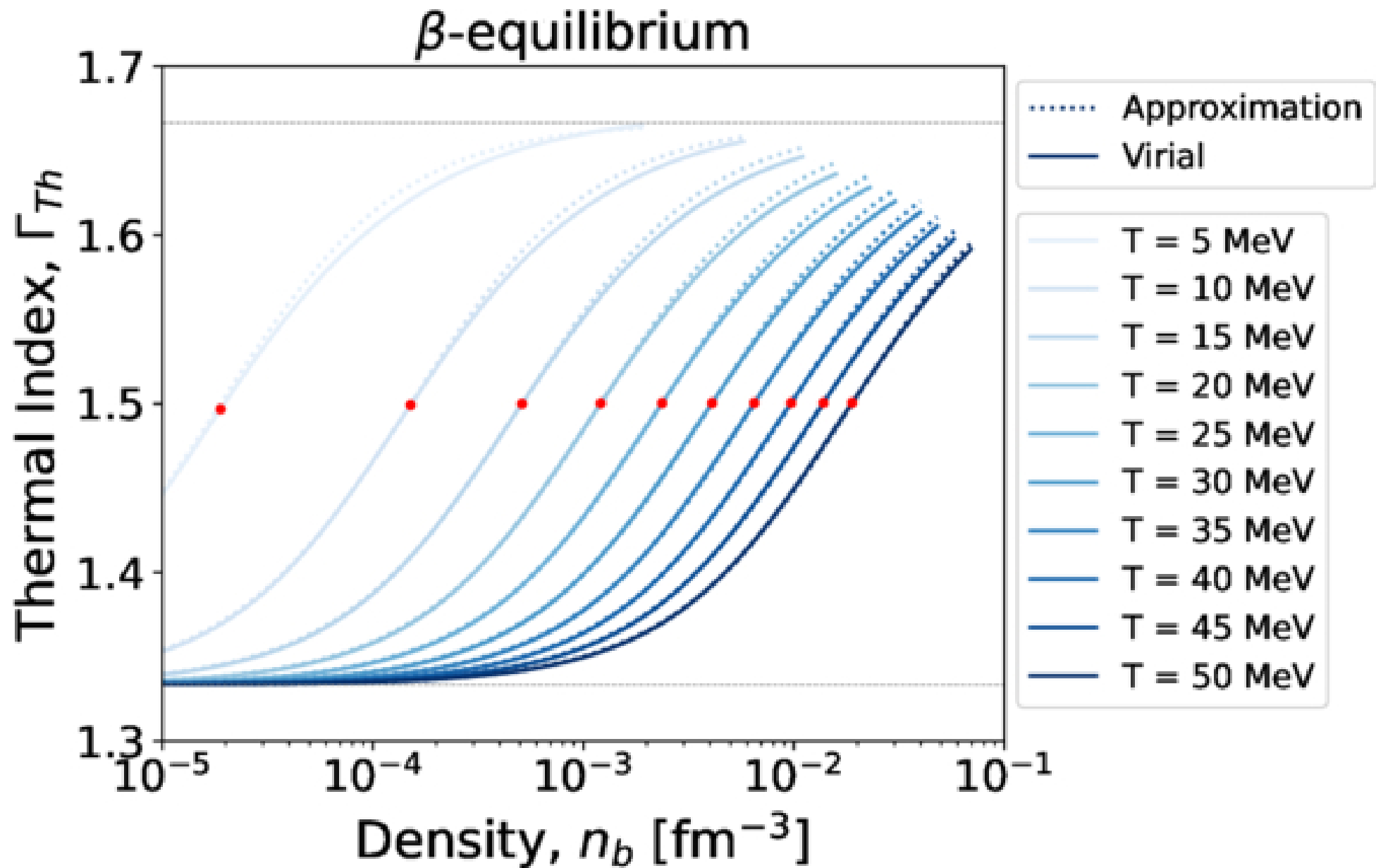
Figure 5. from Giuseppe Riveccio et al 2025 Astrophys. J. 987 doi:10.3847/1538-4357/add3ed https://dx.doi.org/10.3847/1538-4357/add3ed © 2025. The Author(s). Published by the American Astronomical Society.
