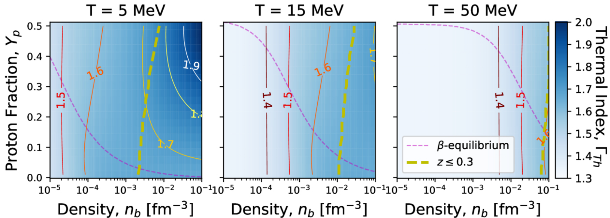
Figure 4. from Giuseppe Riveccio et al 2025 Astrophys. J. 987 doi:10.3847/1538-4357/add3ed https://dx.doi.org/10.3847/1538-4357/add3ed © 2025. The Author(s). Published by the American Astronomical Society.
