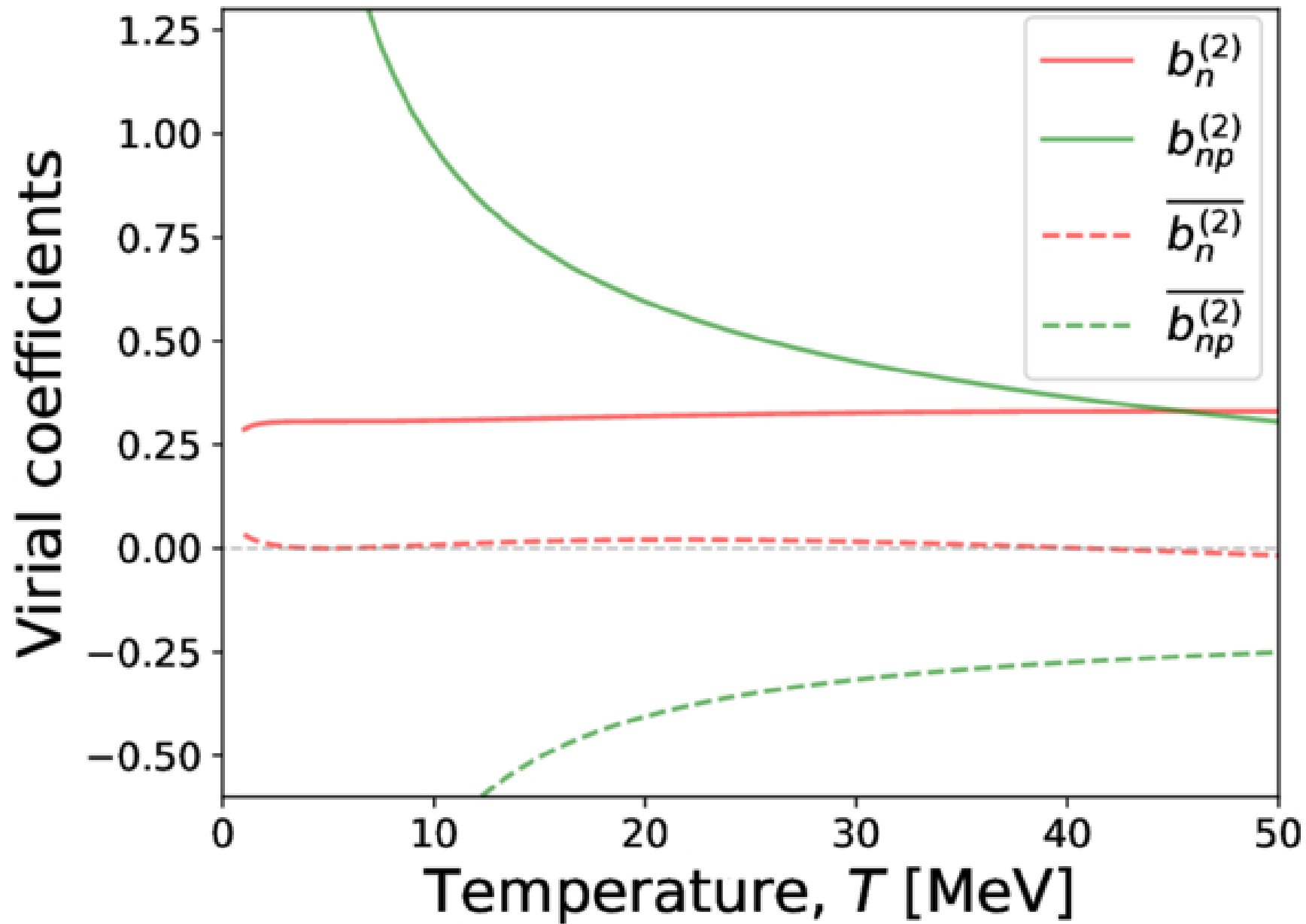
Figure 1. from Giuseppe Riveccio et al 2025 Astrophys. J. 987 doi:10.3847/1538-4357/add3ed https://dx.doi.org/10.3847/1538-4357/add3ed © 2025. The Author(s). Published by the American Astronomical Society.
