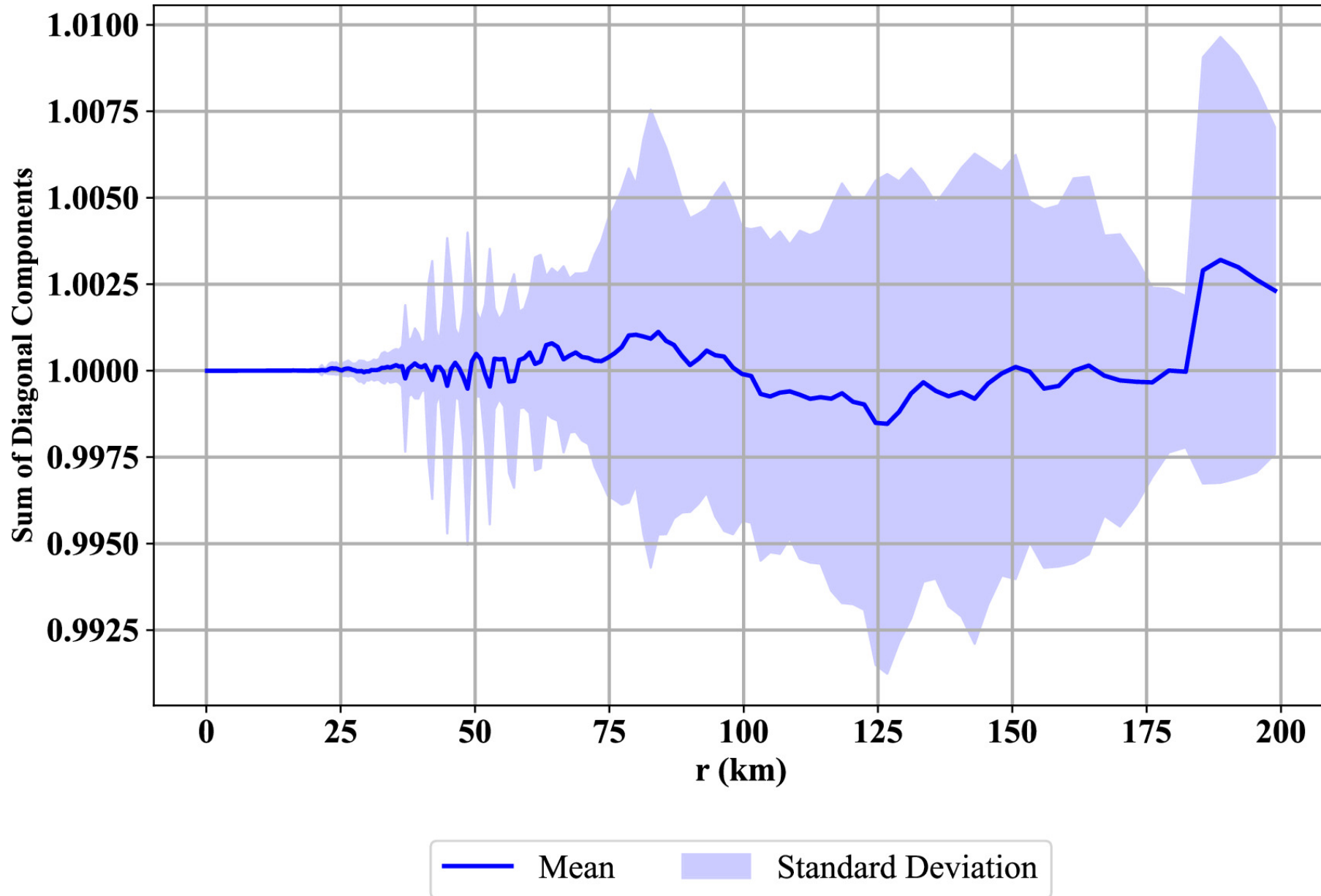
Figure 7. from Shota Takahashi et al 2025 Astrophys. J. 986 doi:10.3847/1538-4357/add0ae https://dx.doi.org/10.3847/1538-4357/add0ae © 2025. The Author(s). Published by the American Astronomical Society.
