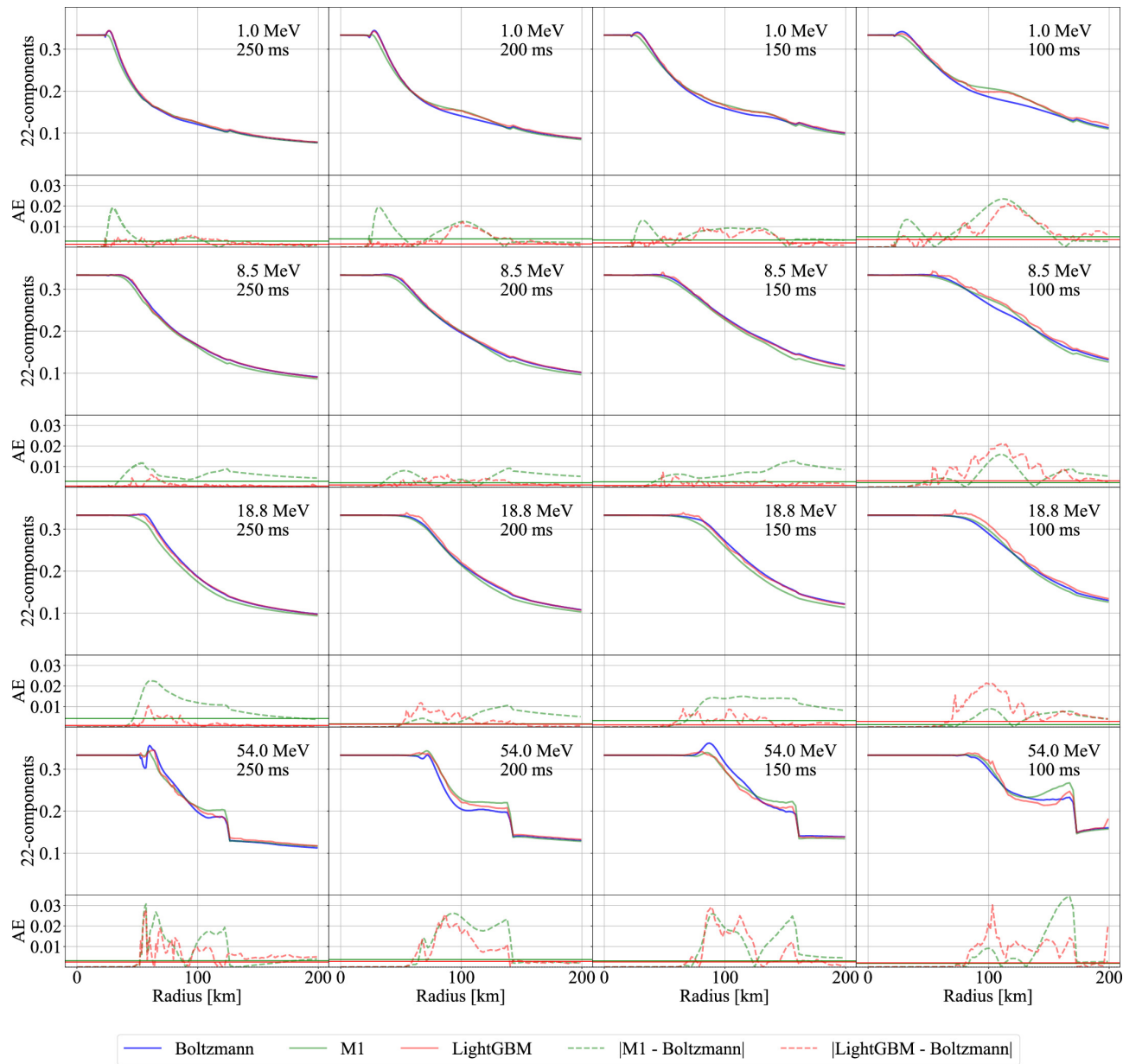
Figure 5. from Shota Takahashi et al 2025 Astrophys. J. 986 doi:10.3847/1538-4357/add0ae https://dx.doi.org/10.3847/1538-4357/add0ae © 2025. The Author(s). Published by the American Astronomical Society.
