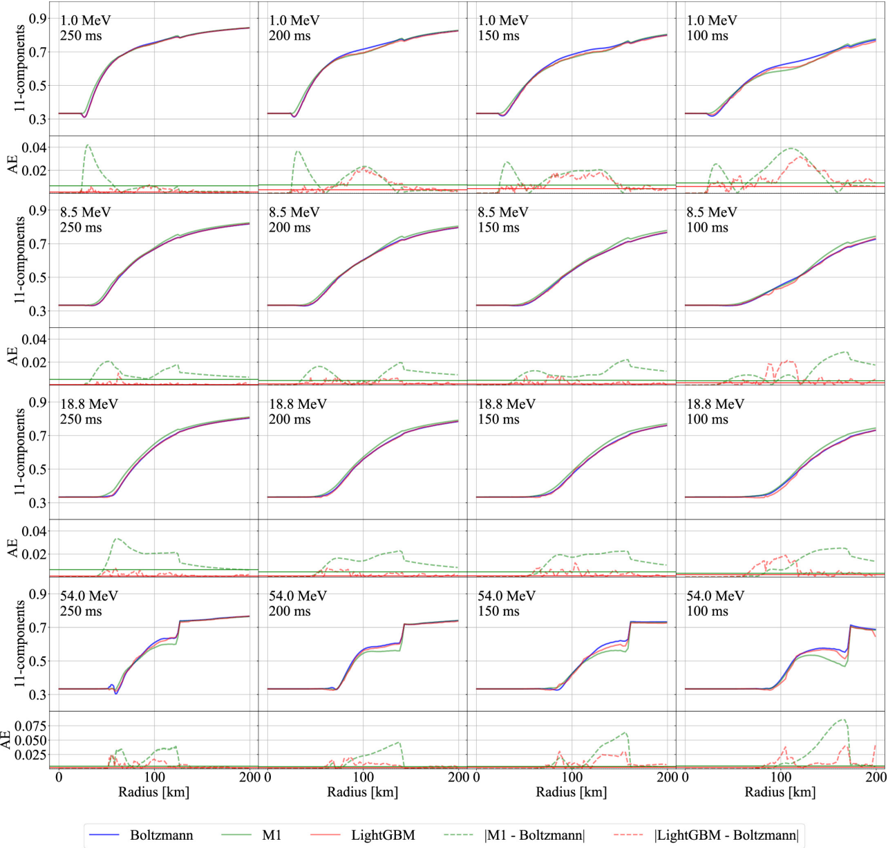
Figure 4. from Shota Takahashi et al 2025 Astrophys. J. 986 doi:10.3847/1538-4357/add0ae https://dx.doi.org/10.3847/1538-4357/add0ae © 2025. The Author(s). Published by the American Astronomical Society.
