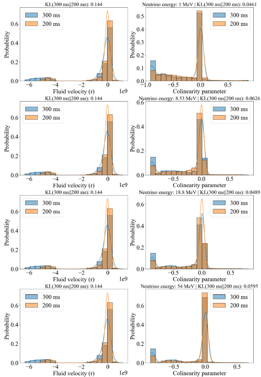
Figure 11. from Shota Takahashi et al 2025 Astrophys. J. 986 doi:10.3847/1538-4357/add0ae https://dx.doi.org/10.3847/1538-4357/add0ae © 2025. The Author(s). Published by the American Astronomical Society.
