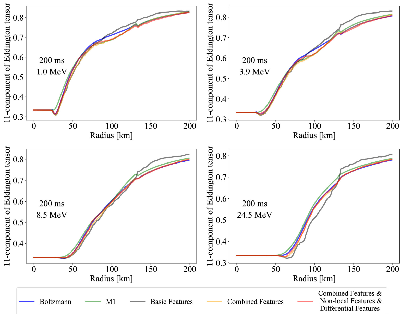
Figure 10. from Shota Takahashi et al 2025 Astrophys. J. 986 doi:10.3847/1538-4357/add0ae https://dx.doi.org/10.3847/1538-4357/add0ae © 2025. The Author(s). Published by the American Astronomical Society.
