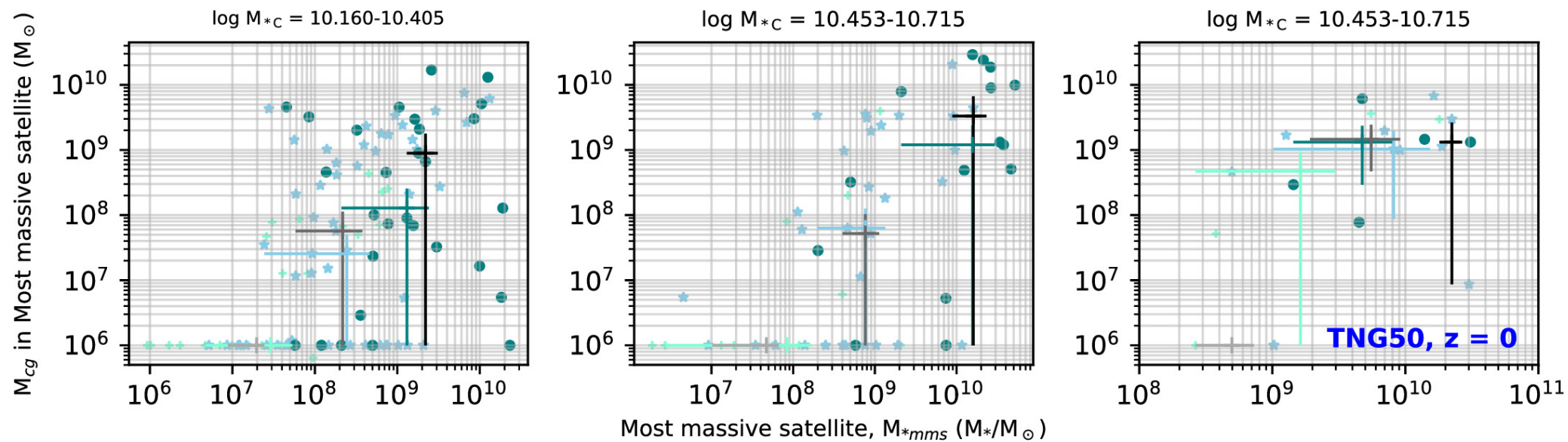
Figure 6. from Mitali Damle et al 2025 Astrophys. J. 986 doi:10.3847/1538-4357/adcee9 https://dx.doi.org/10.3847/1538-4357/adcee9 © 2025. The Author(s). Published by the American Astronomical Society.
